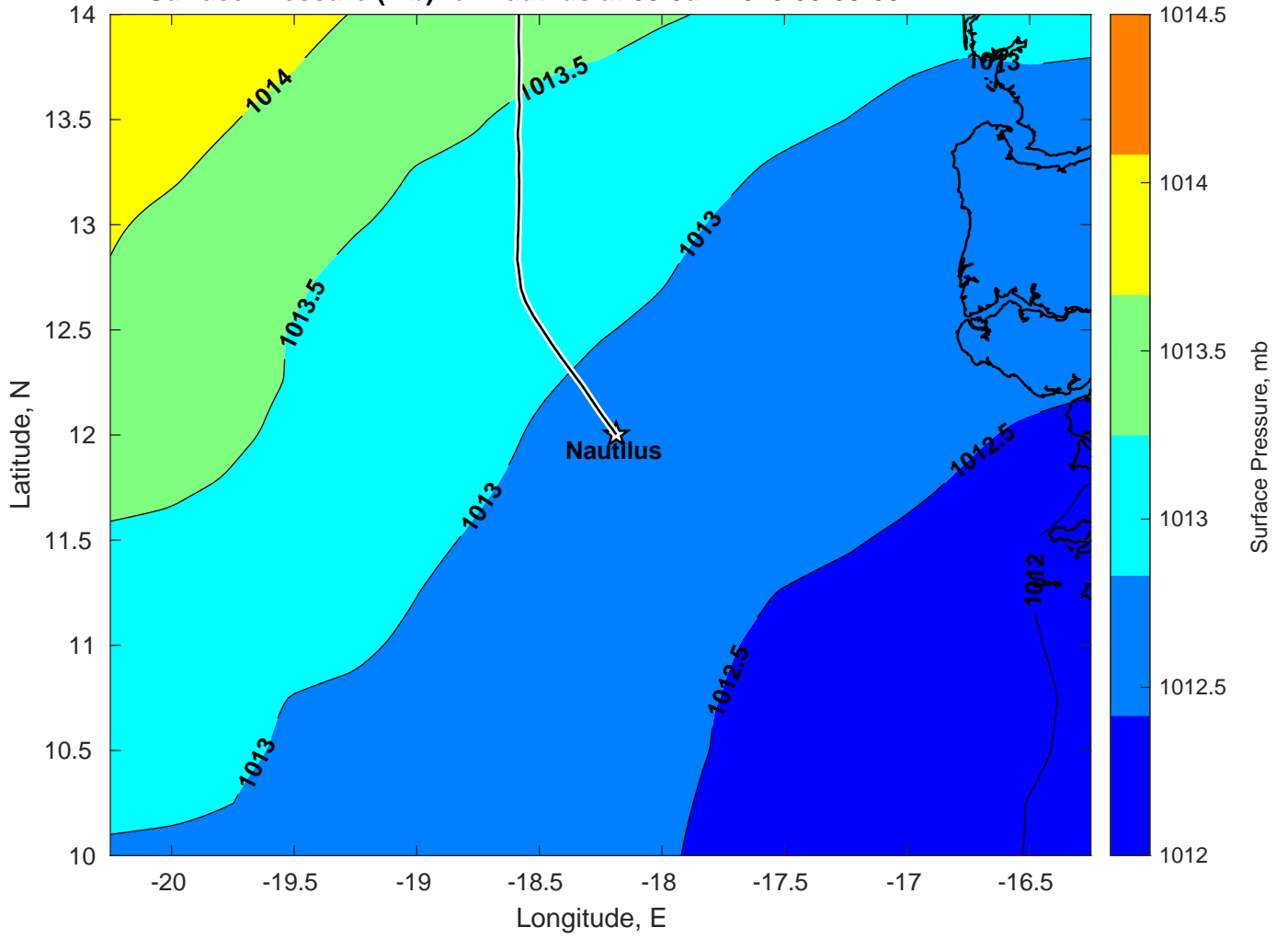
Surface Pressure (mb) for Nautilus at 03-Jan-2025 00:00:00
