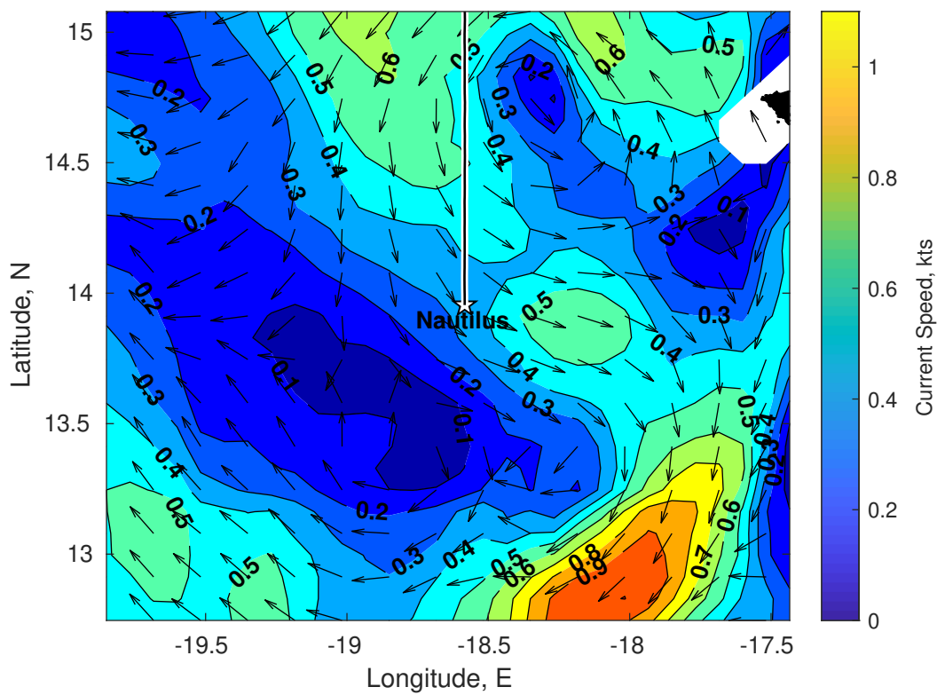
Surface Currents for Nautilus at 01-Jan-2025 00:00:00
