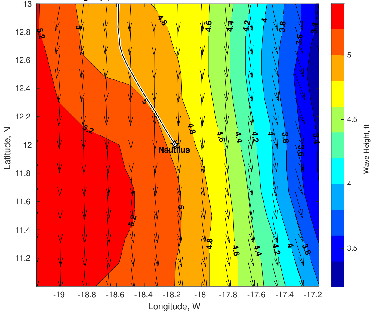
Wave Height (ft) for Nautilus at 02-Jan-2025 09:00:00
