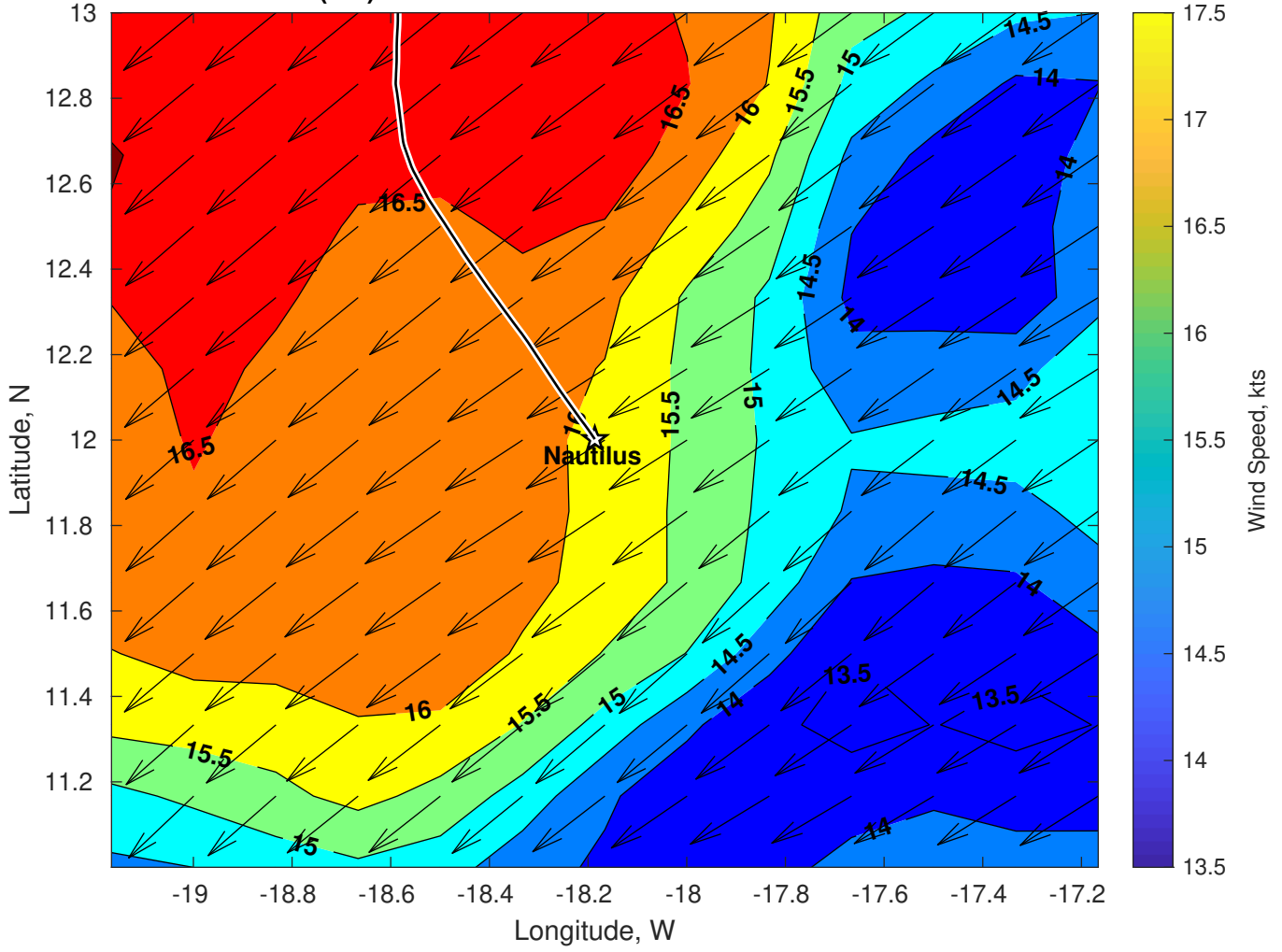
Winds (kts) for Nautilus at 02-Jan-2025 09:00:00
