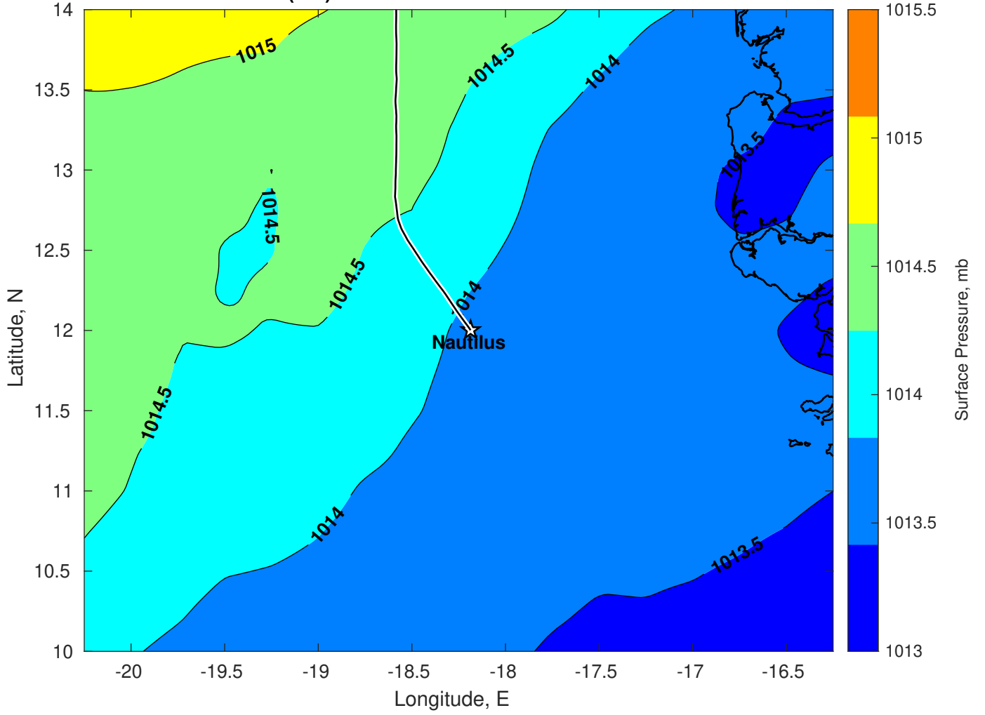
Surface Pressure (mb) for Nautilus at 04-Jan-2025 00:00:00
