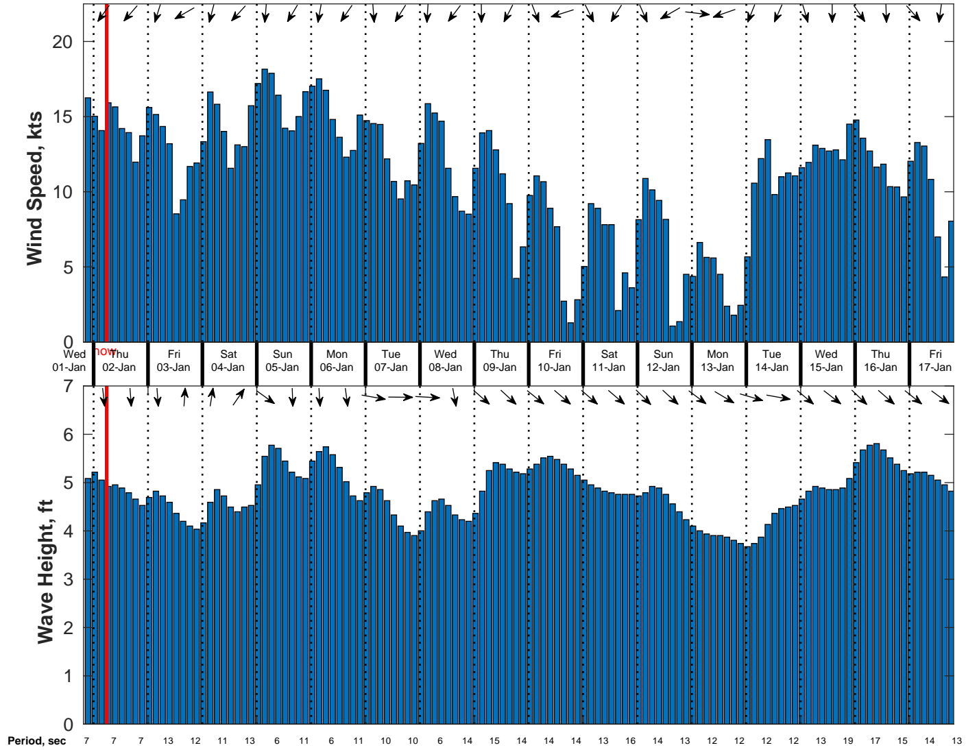
Wind & Wave Forecast for Nautilus from 01-Jan-2025 20:00:00 to 17-Jan-2025 20:00:00
