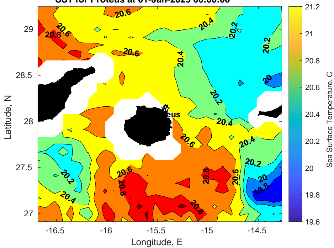
SST for Proteus at 01-Jan-2025 00:00:00
