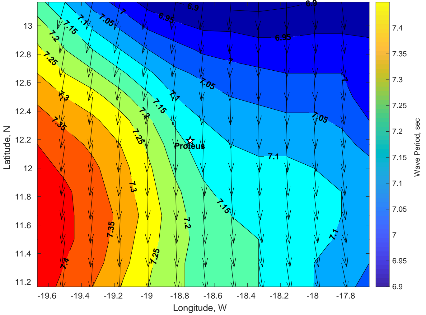
Wave Period (sec) for Proteus at 02-Jan-2025 09:00:00
