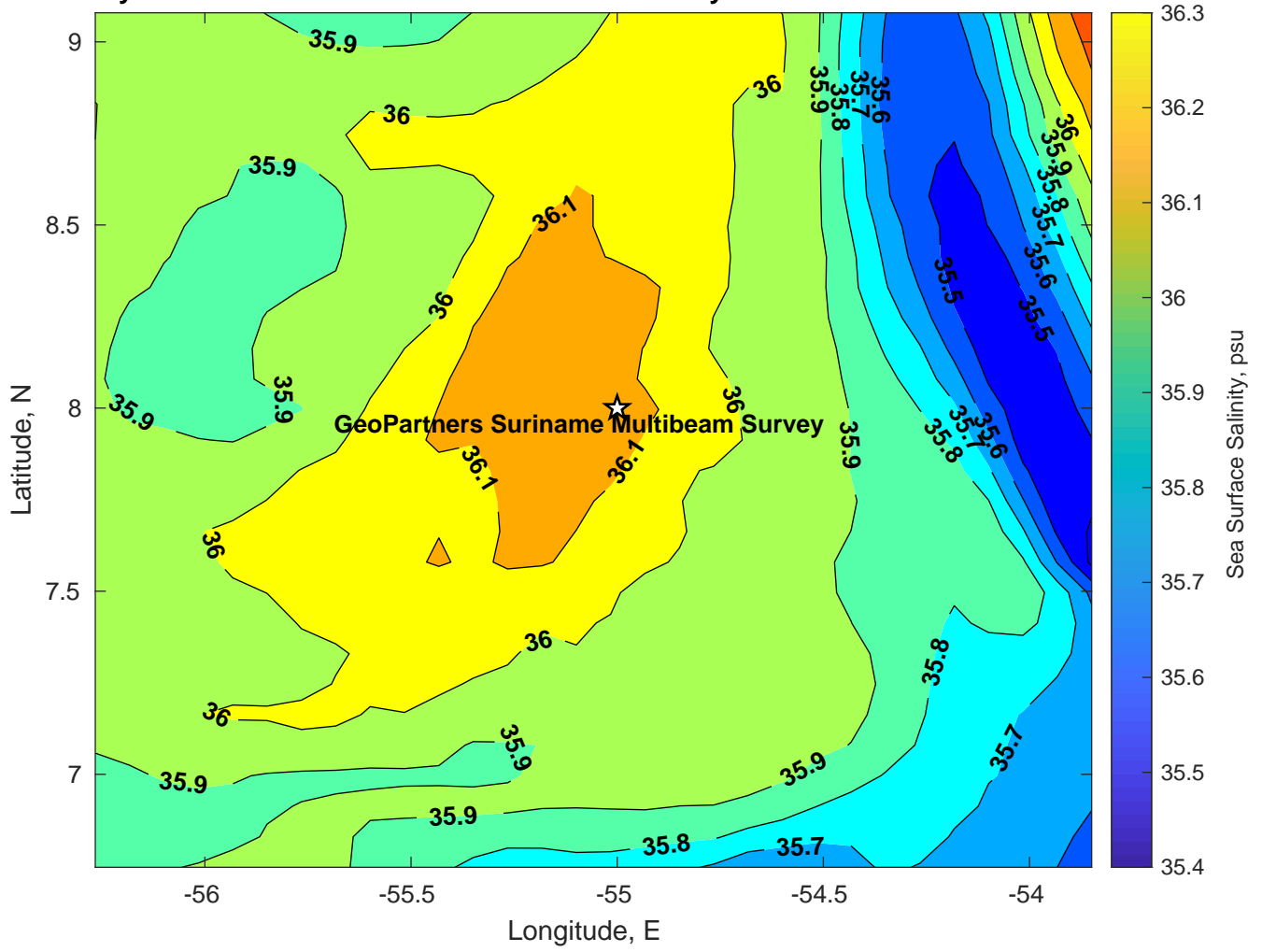
Surface Salinity for GeoPartners Suriname Multibeam Survey at 02-Jan-2025 00:00:00
