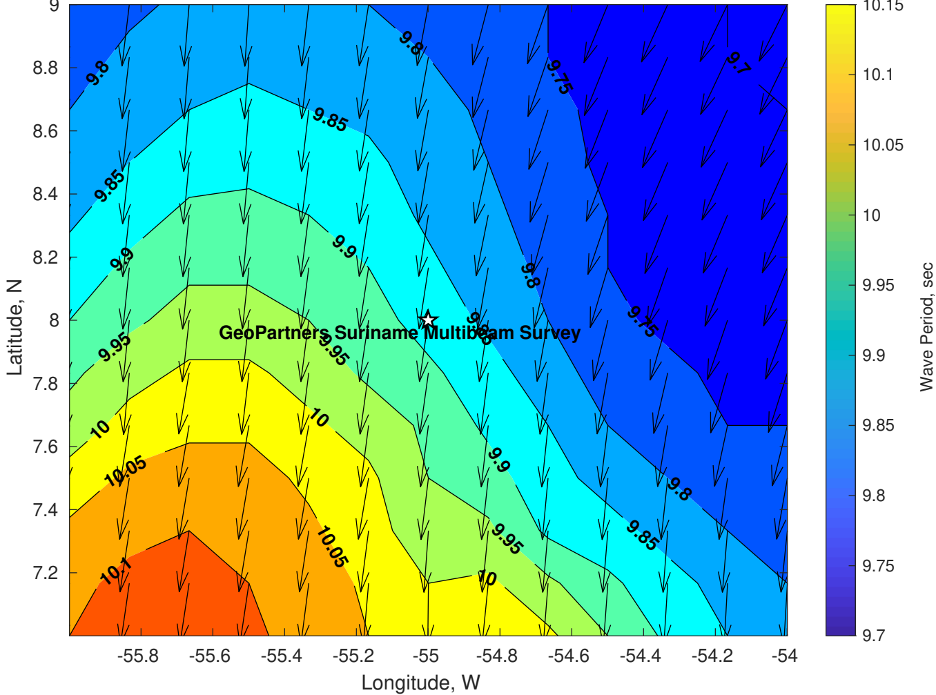
Wave Period (sec) for GeoPartners Suriname Multibeam Survey at 02-Jan-2025 21:00:00
