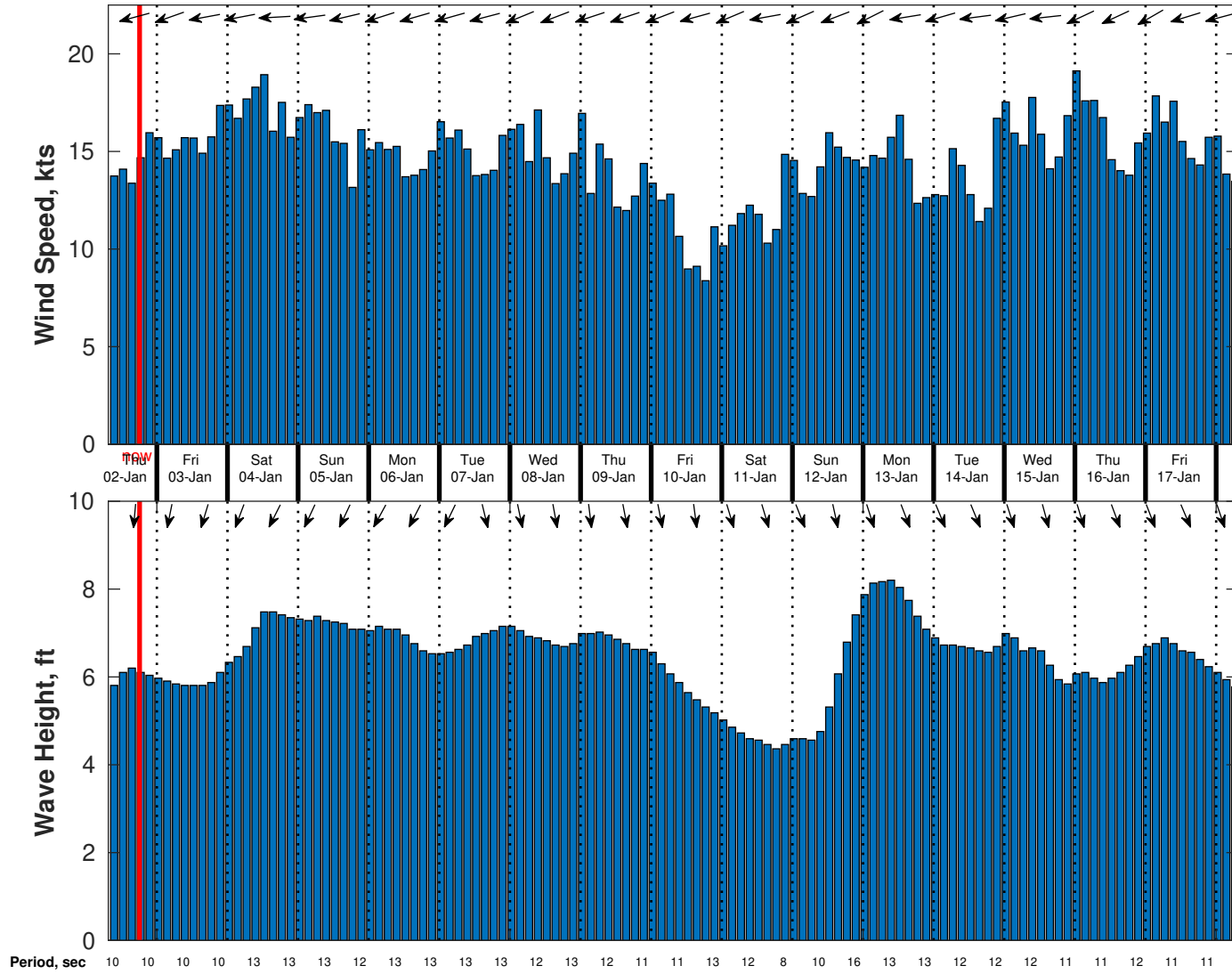
Wind & Wave Forecast for GeoPartners Suriname Multibeam Survey from 02-Jan-2025 08:00:00 to 18-Jan-2025 08:00:00
