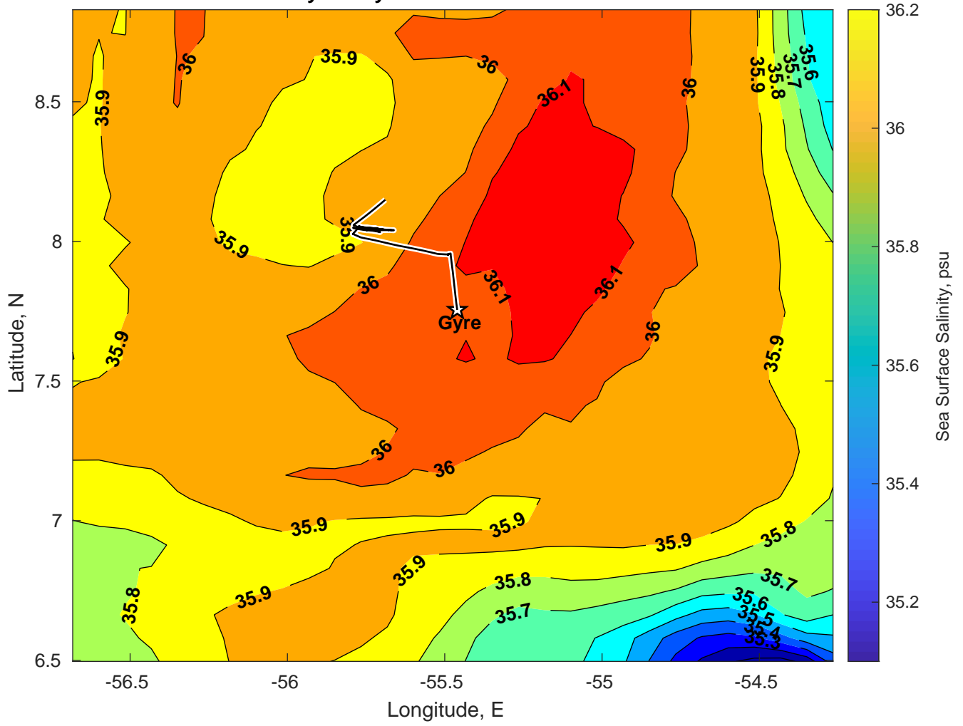
Surface Salinity for Gyre at 02-Jan-2025 00:00:00
