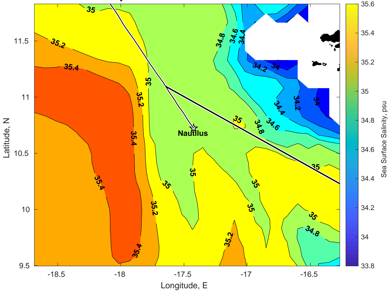
Surface Salinity for Nautilus at 02-Jan-2025 00:00:00
