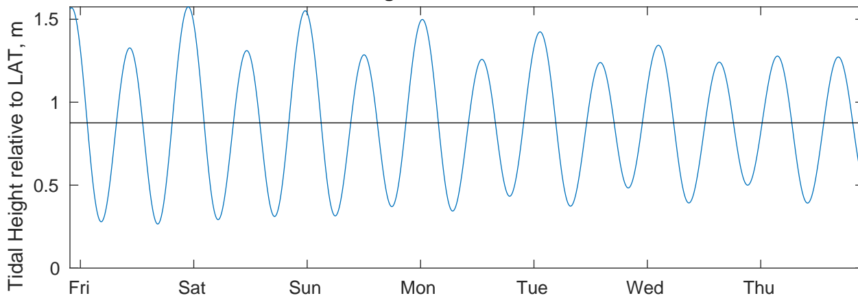
Tidal Currents and Heights for Nautilus at 20250102
