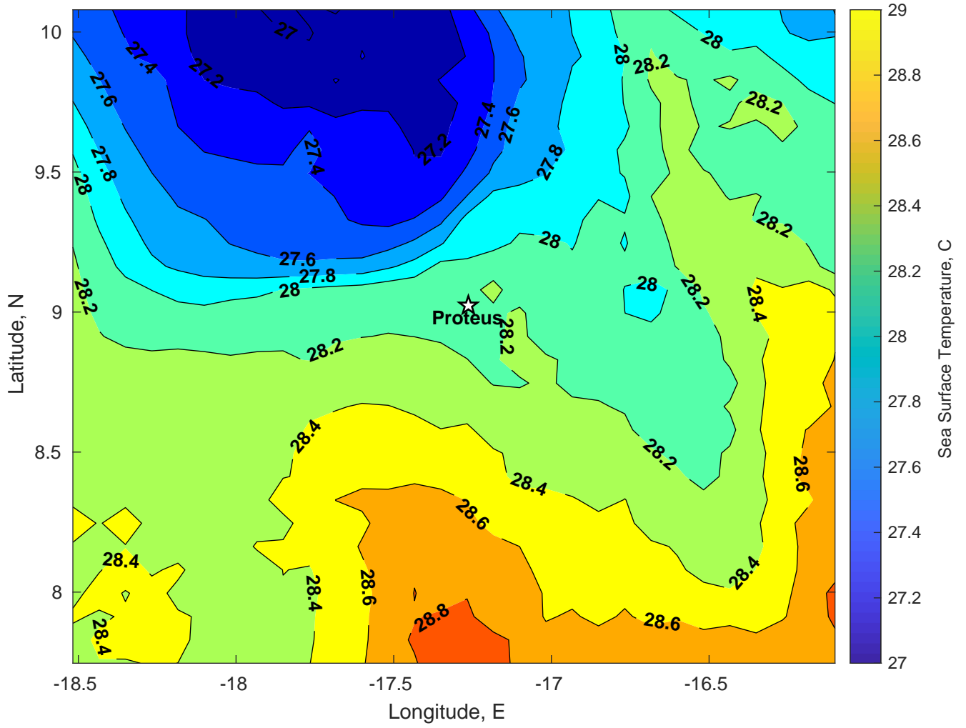
SST for Proteus at 02-Jan-2025 00:00:00
