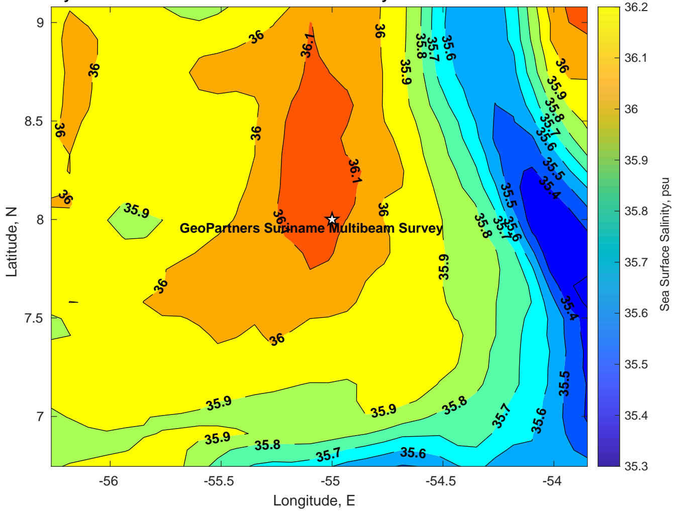
Surface Salinity for GeoPartners Suriname Multibeam Survey at 03-Jan-2025 00:00:00
