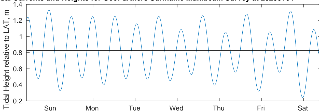
Tidal Currents and Heights for GeoPartners Suriname Multibeam Survey at 20250104
