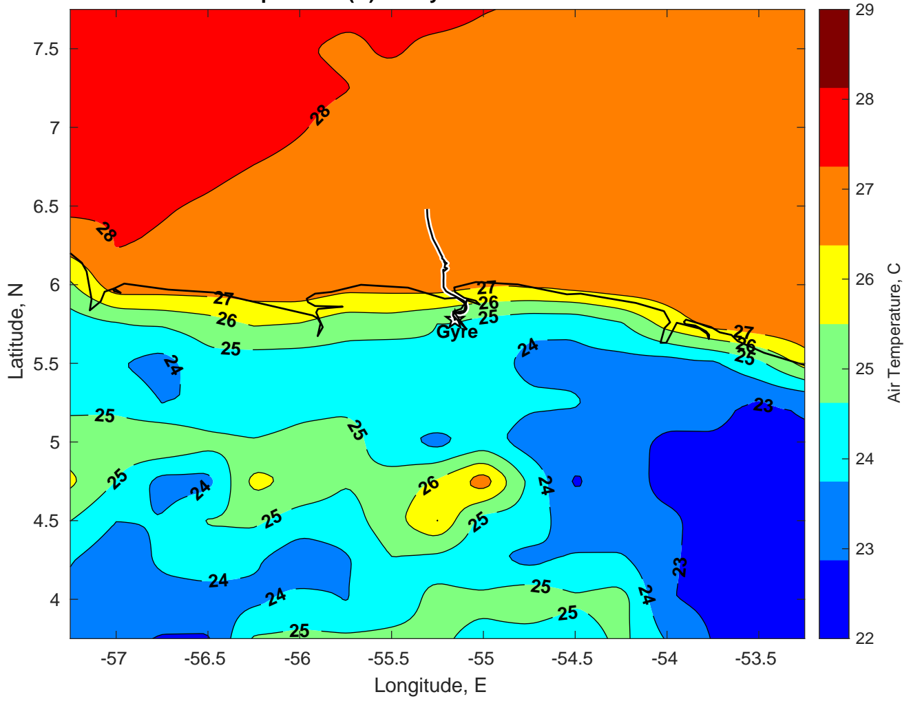
Air Temperature (C) for Gyre at 04-Jan-2025
