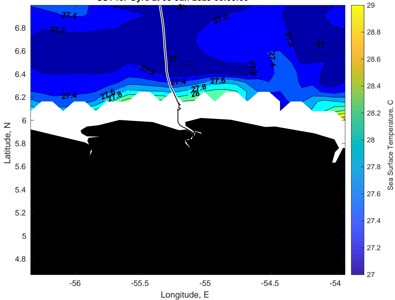
SST for Gyre at 03-Jan-2025 00:00:00
