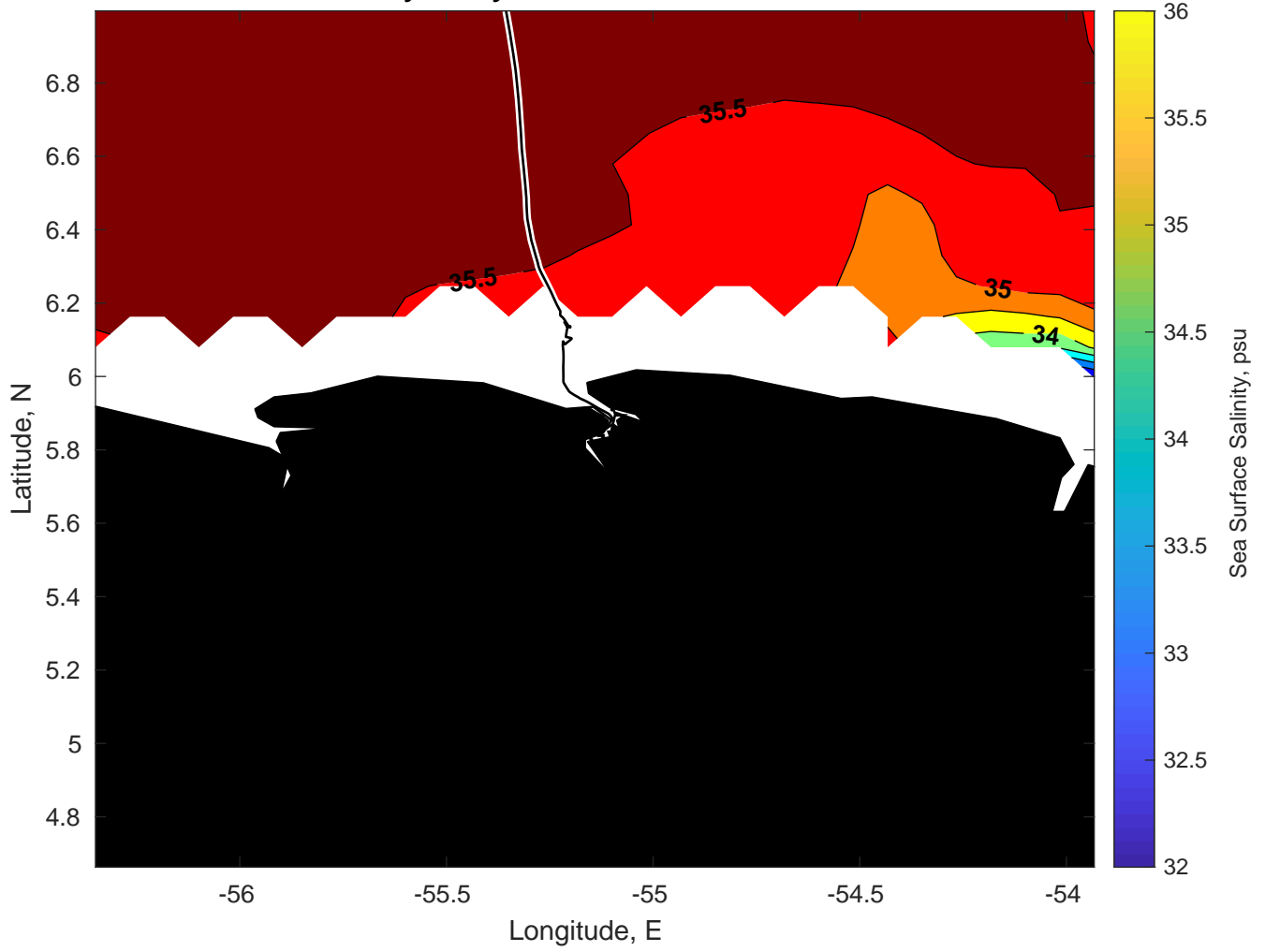
Surface Salinity for Gyre at 03-Jan-2025 00:00:00
