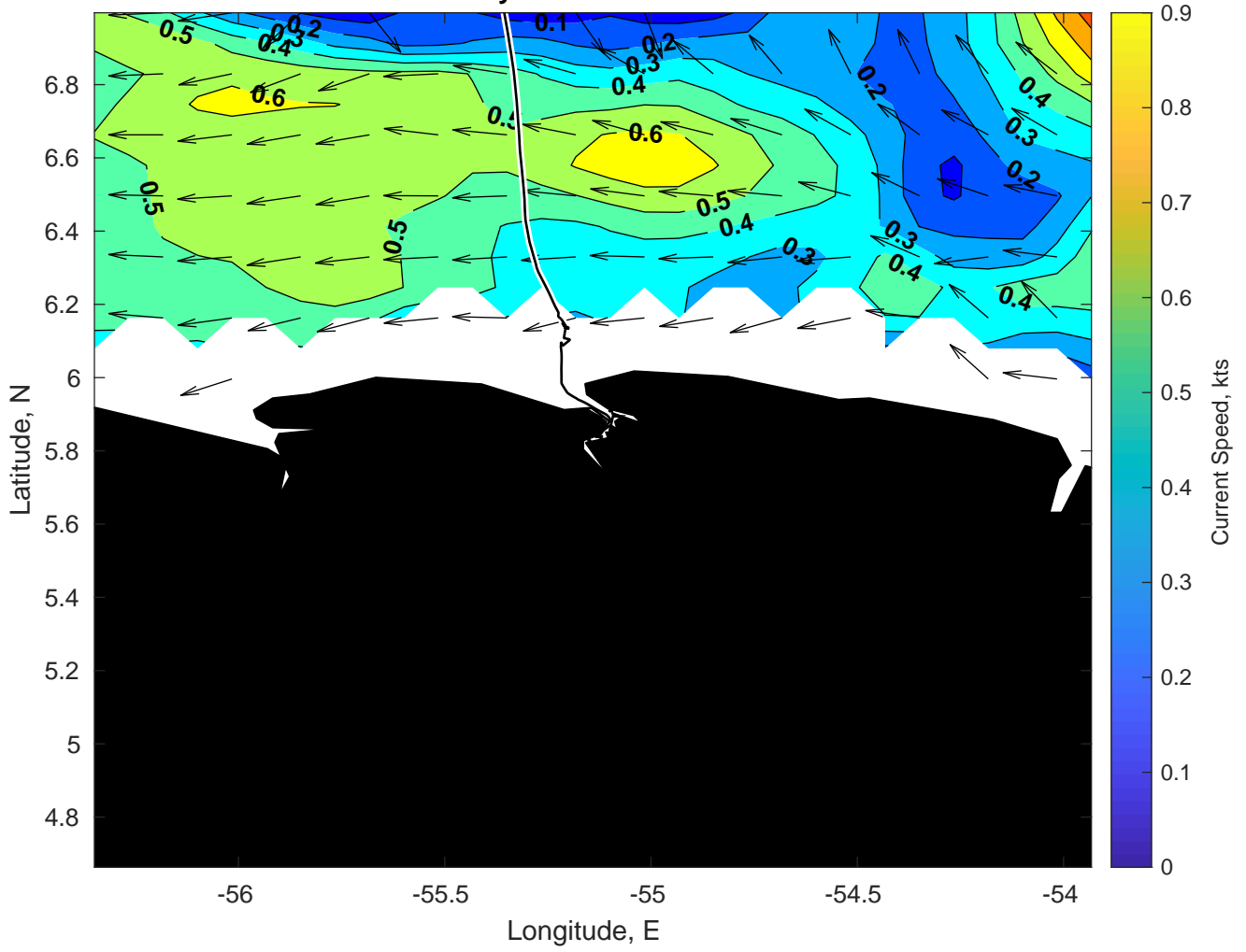
Surface Currents for Gyre at 03-Jan-2025 00:00:00
