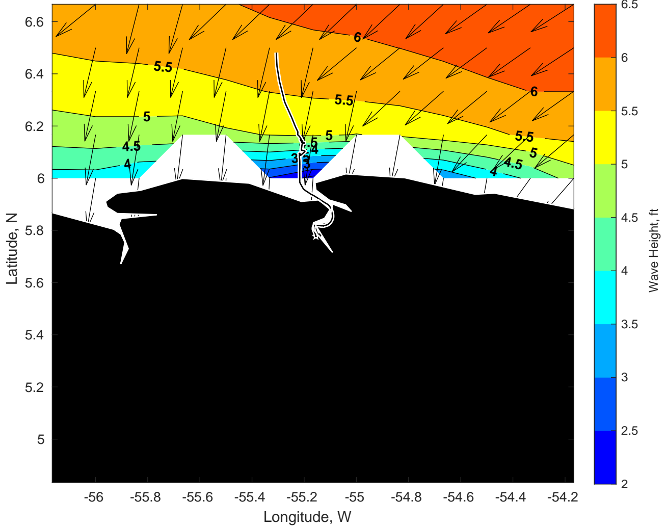
Wave Height (ft) for Gyre at 04-Jan-2025 09:00:00
