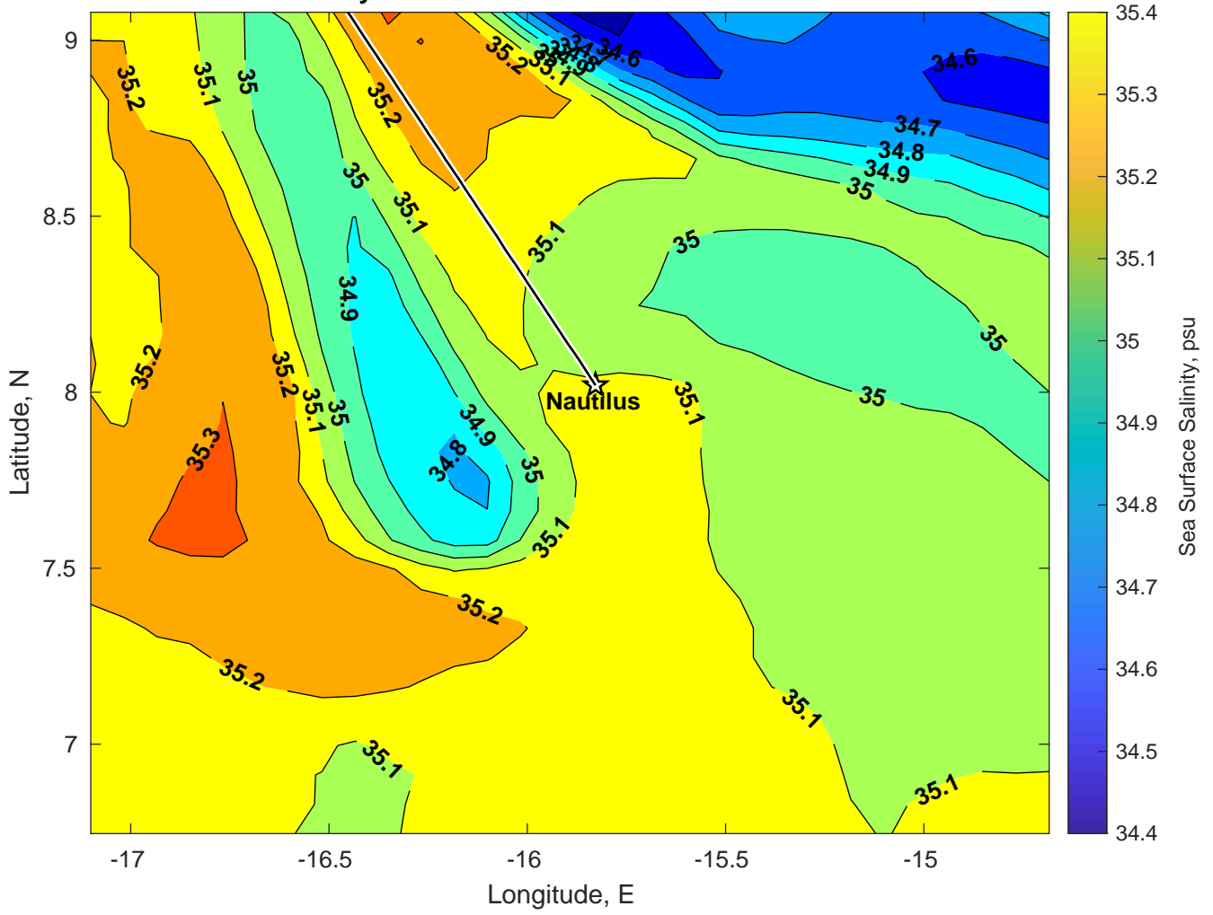
Surface Salinity for Nautilus at 03-Jan-2025 00:00:00
