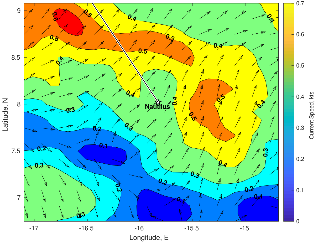
Surface Currents for Nautilus at 03-Jan-2025 00:00:00
