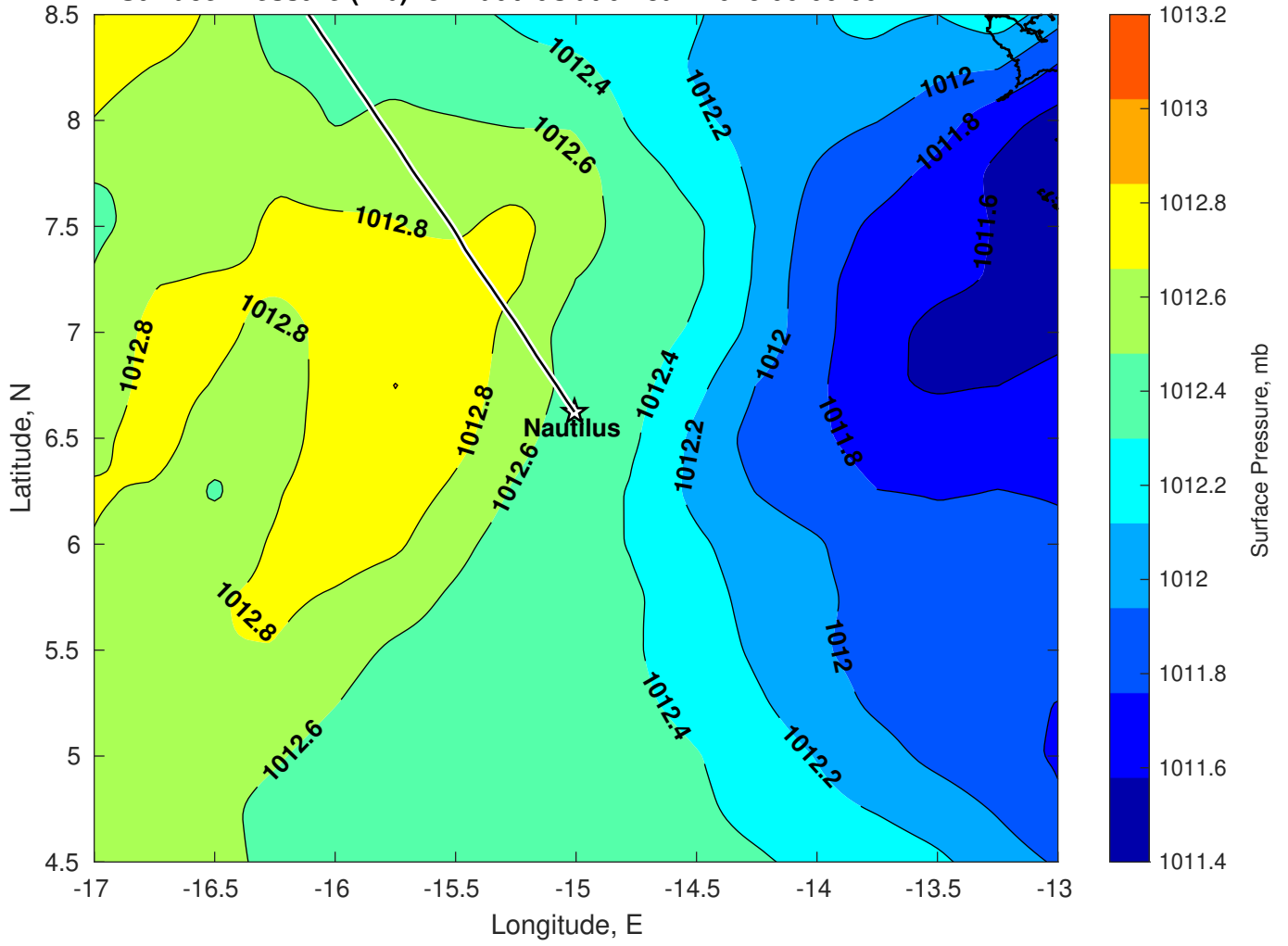
Surface Pressure (mb) for Nautilus at 04-Jan-2025 00:00:00
