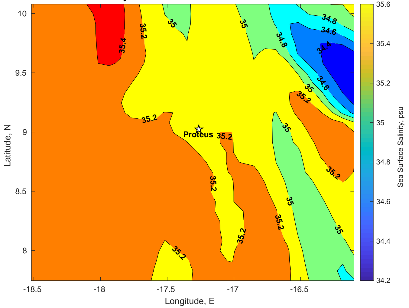
Surface Salinity for Proteus at 03-Jan-2025 00:00:00
