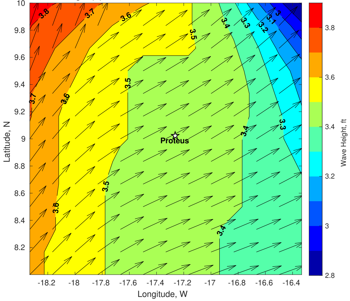
Wave Height (ft) for Proteus at 04-Jan-2025 09:00:00
