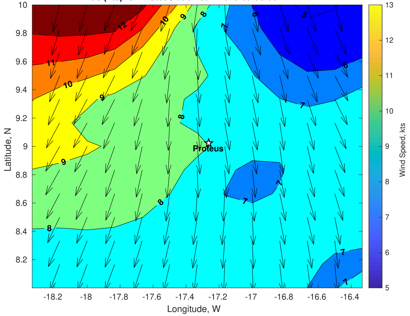
Winds (kts) for Proteus at 04-Jan-2025 09:00:00
