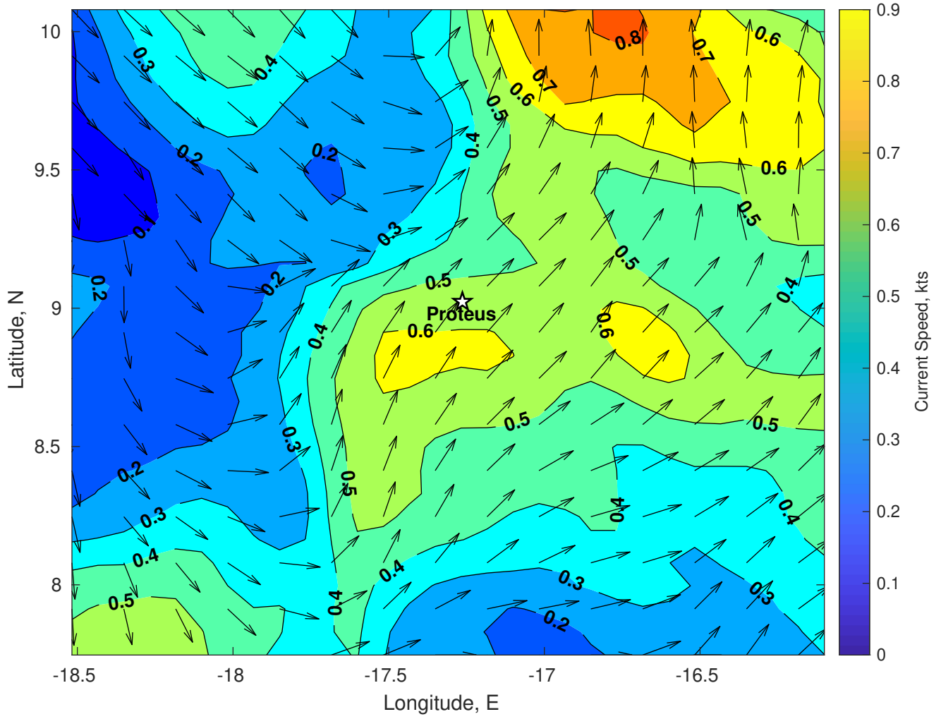
Surface Currents for Proteus at 03-Jan-2025 00:00:00
