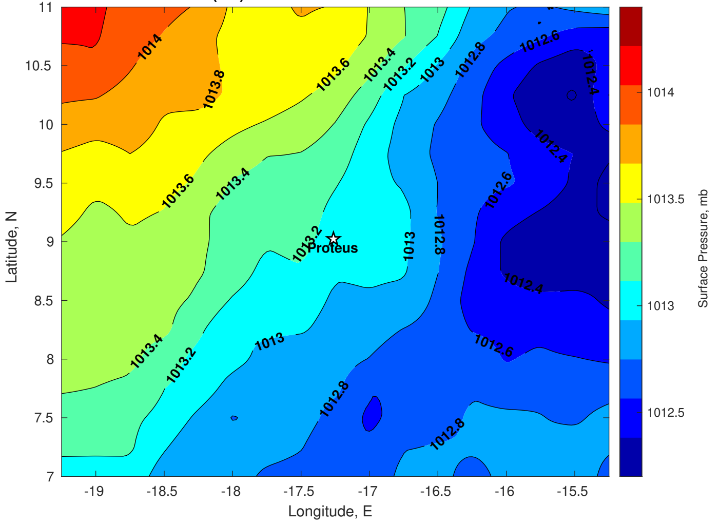
Surface Pressure (mb) for Proteus at 04-Jan-2025 00:00:00
