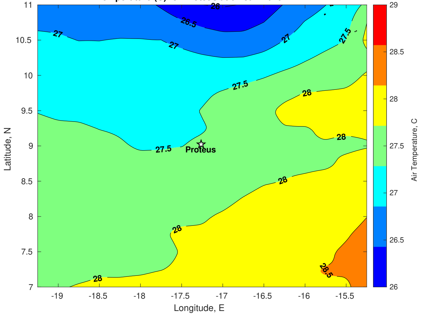
Air Temperature (C) for Proteus at 04-Jan-2025
