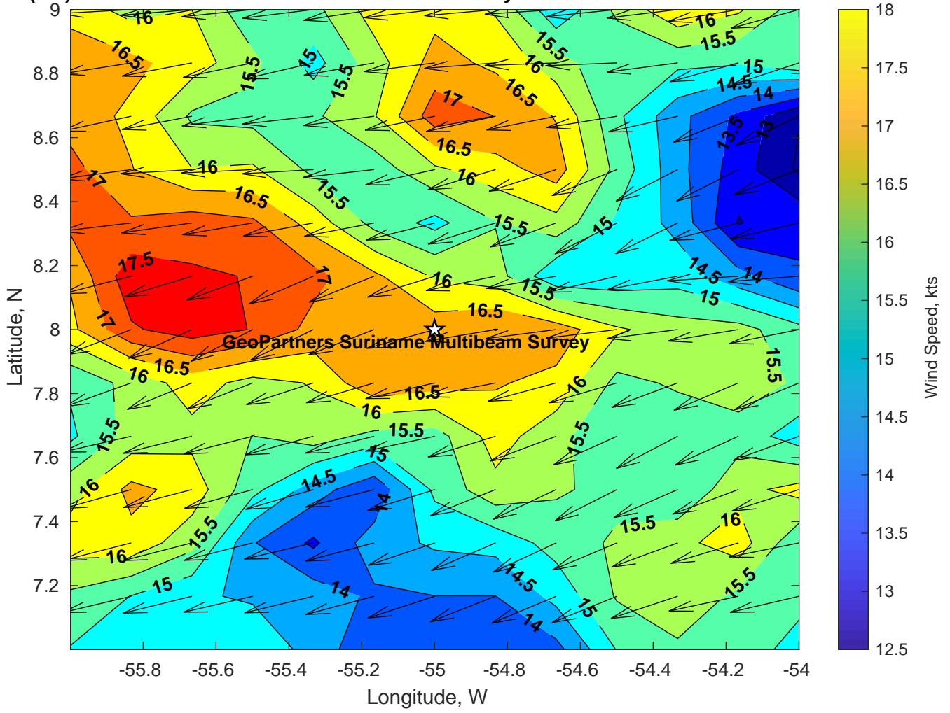
Winds (kts) for GeoPartners Suriname Multibeam Survey at 05-Jan-2025 09:00:00
