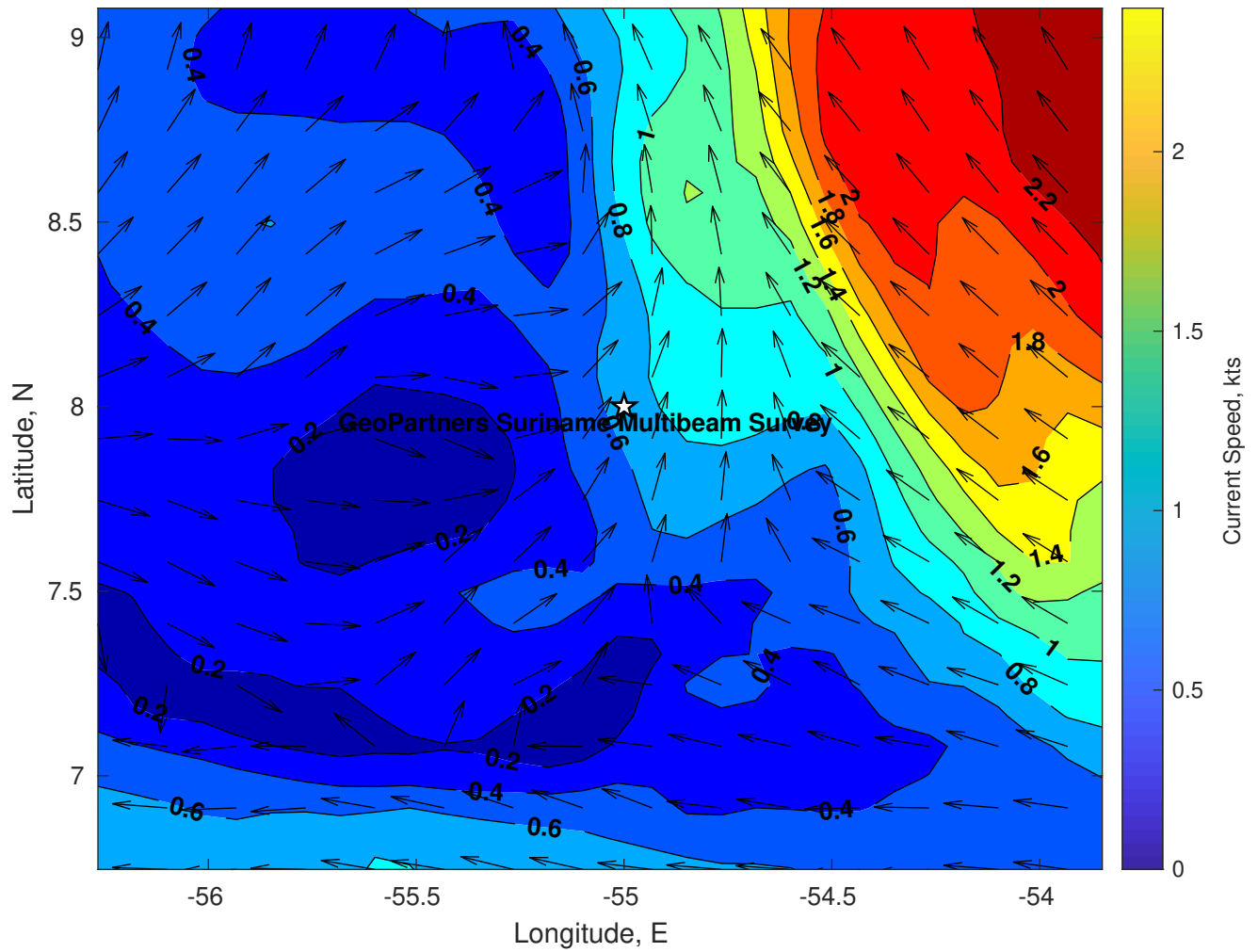
Surface Currents for GeoPartners Suriname Multibeam Survey at 04-Jan-2025 00:00:00
