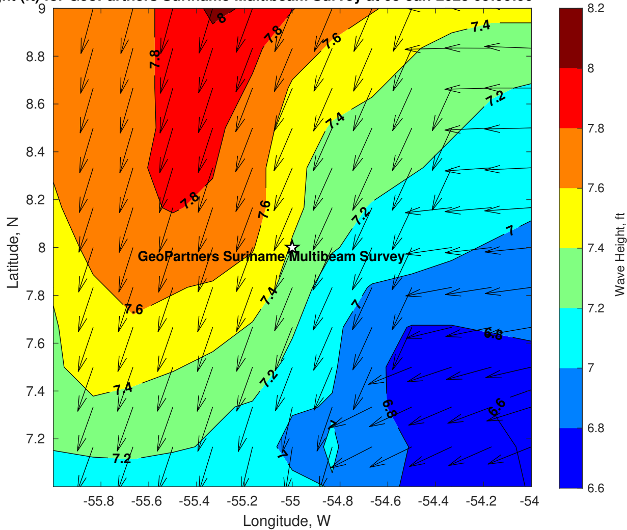
Wave Height (ft) for GeoPartners Suriname Multibeam Survey at 05-Jan-2025 09:00:00
