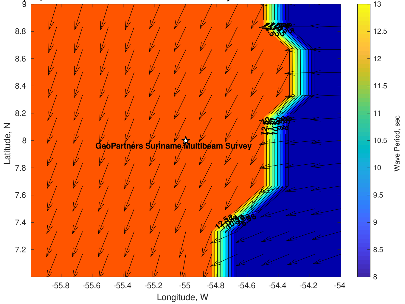
Wave Period (sec) for GeoPartners Suriname Multibeam Survey at 05-Jan-2025 09:00:00
