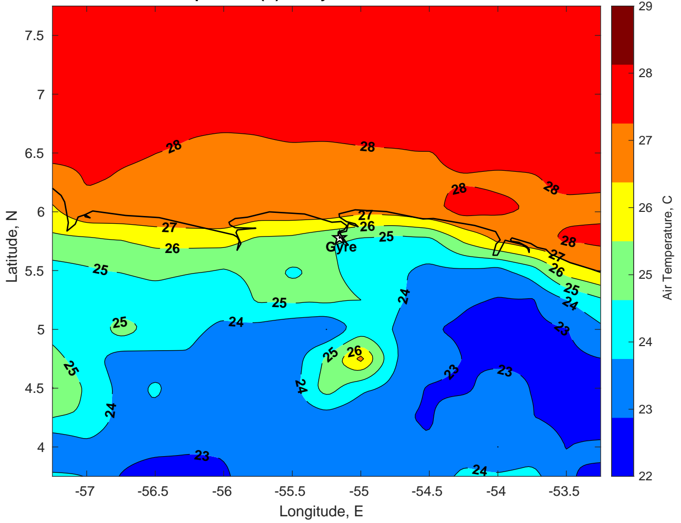
Air Temperature (C) for Gyre at 05-Jan-2025
