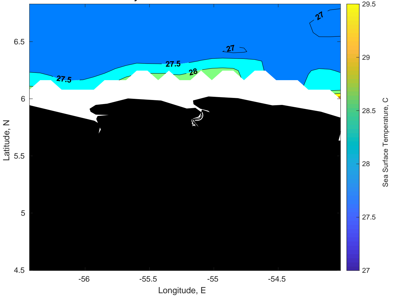
SST for Gyre at 04-Jan-2025 00:00:00
