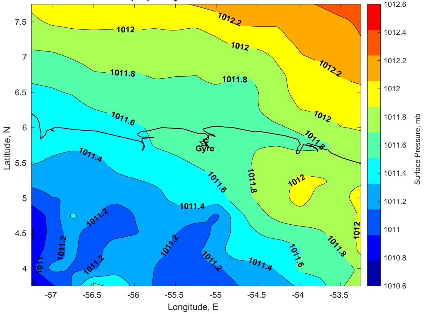
Surface Pressure (mb) for Gyre at 05-Jan-2025 00:00:00
