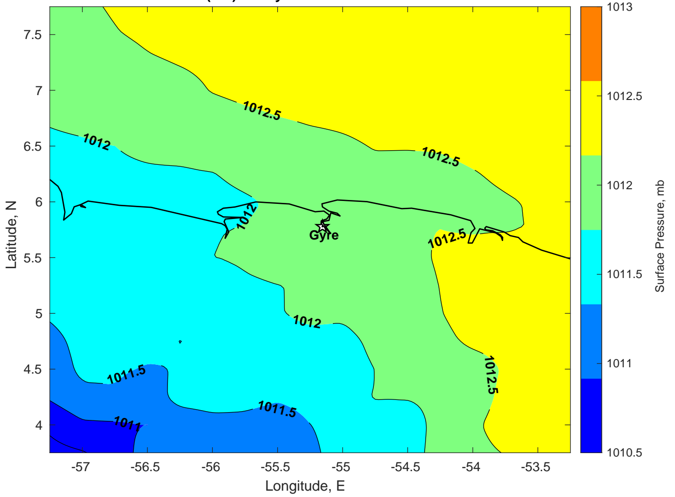
Surface Pressure (mb) for Gyre at 07-Jan-2025 00:00:00
