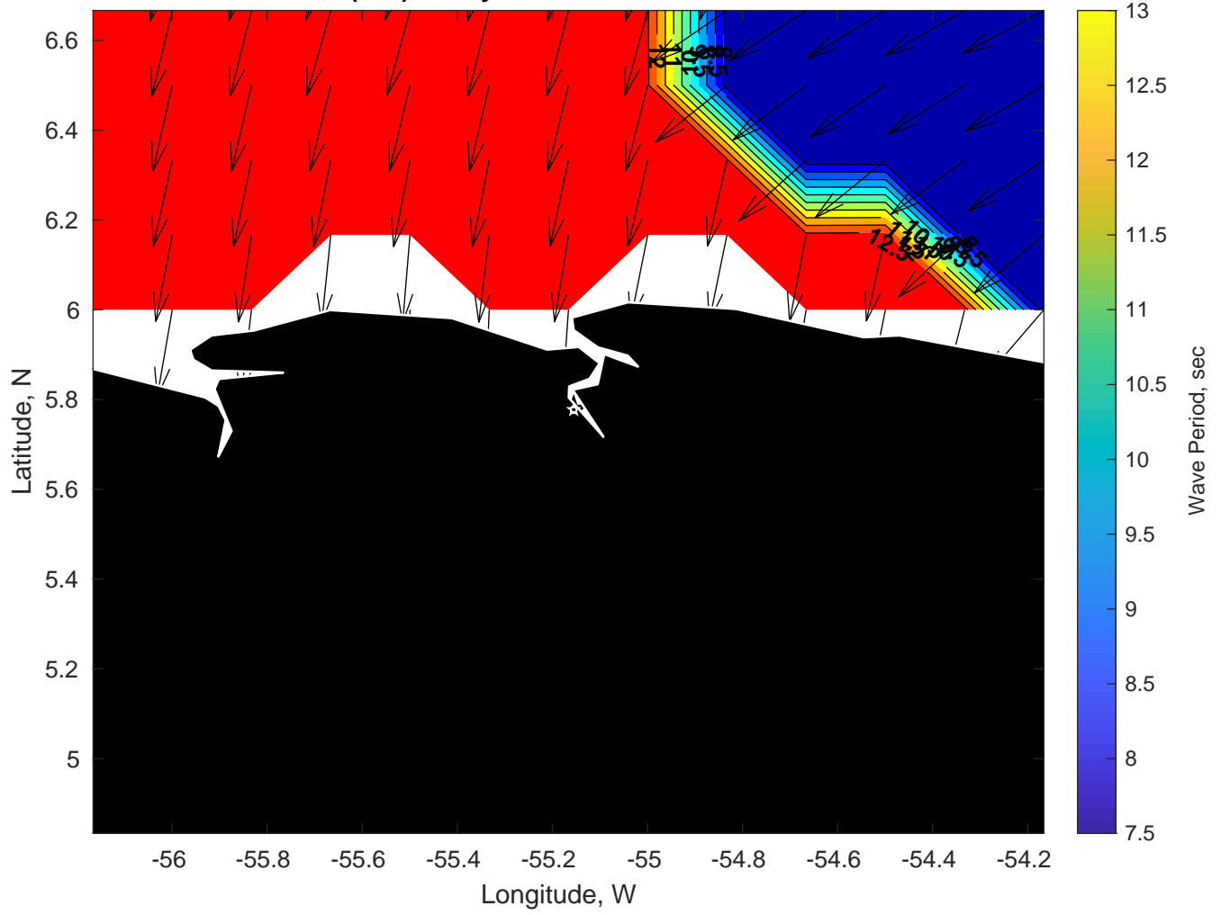
Wave Period (sec) for Gyre at 05-Jan-2025 09:00:00
