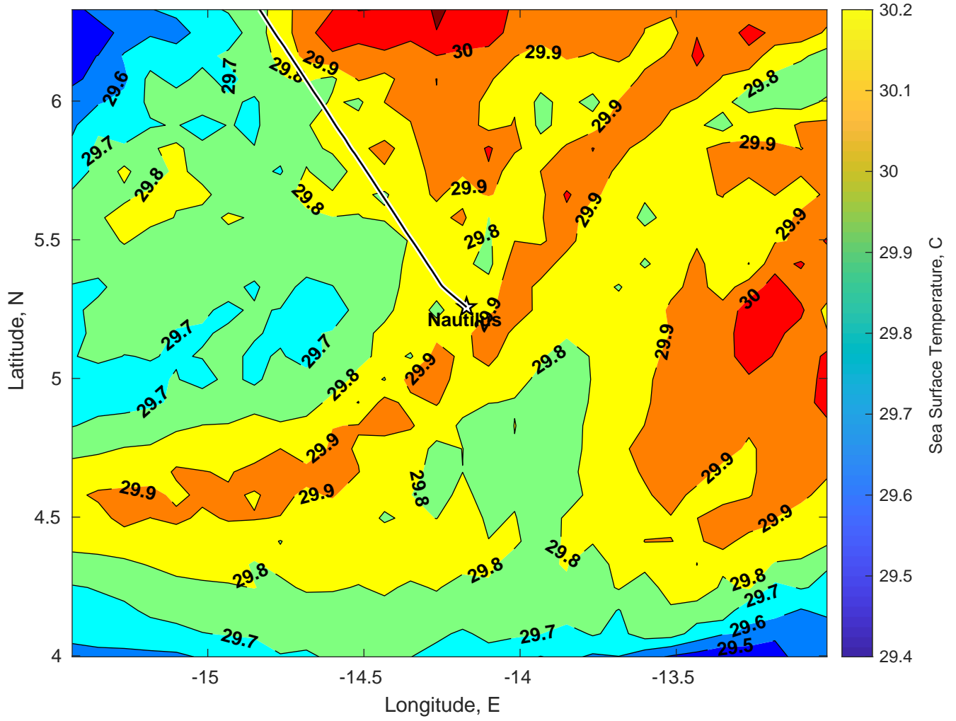
SST for Nautilus at 04-Jan-2025 00:00:00
