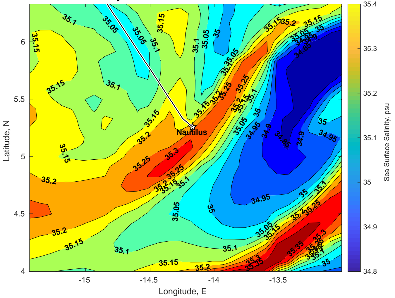
Surface Salinity for Nautilus at 04-Jan-2025 00:00:00
