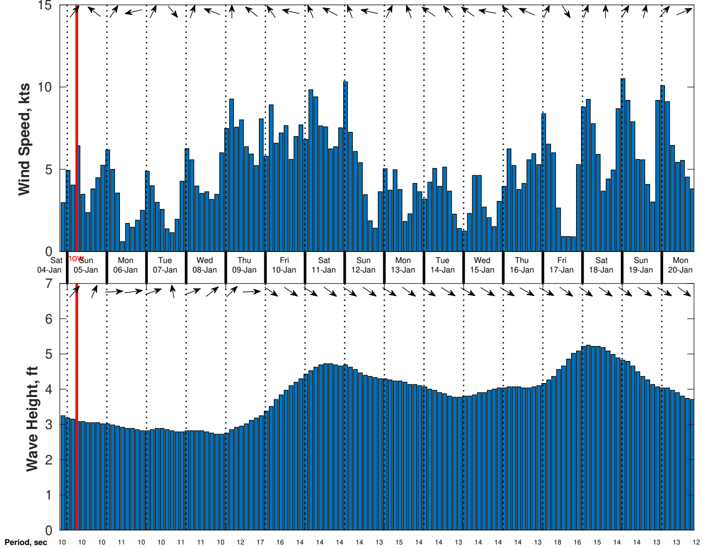
Wind & Wave Forecast for Nautilus from 04-Jan-2025 20:00:00 to 20-Jan-2025 20:00:00
