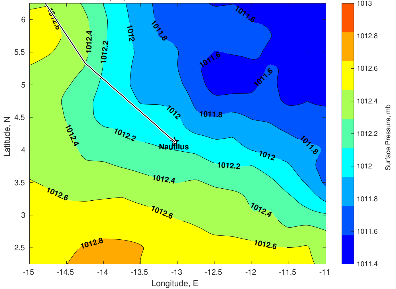
Surface Pressure (mb) for Nautilus at 05-Jan-2025 00:00:00
