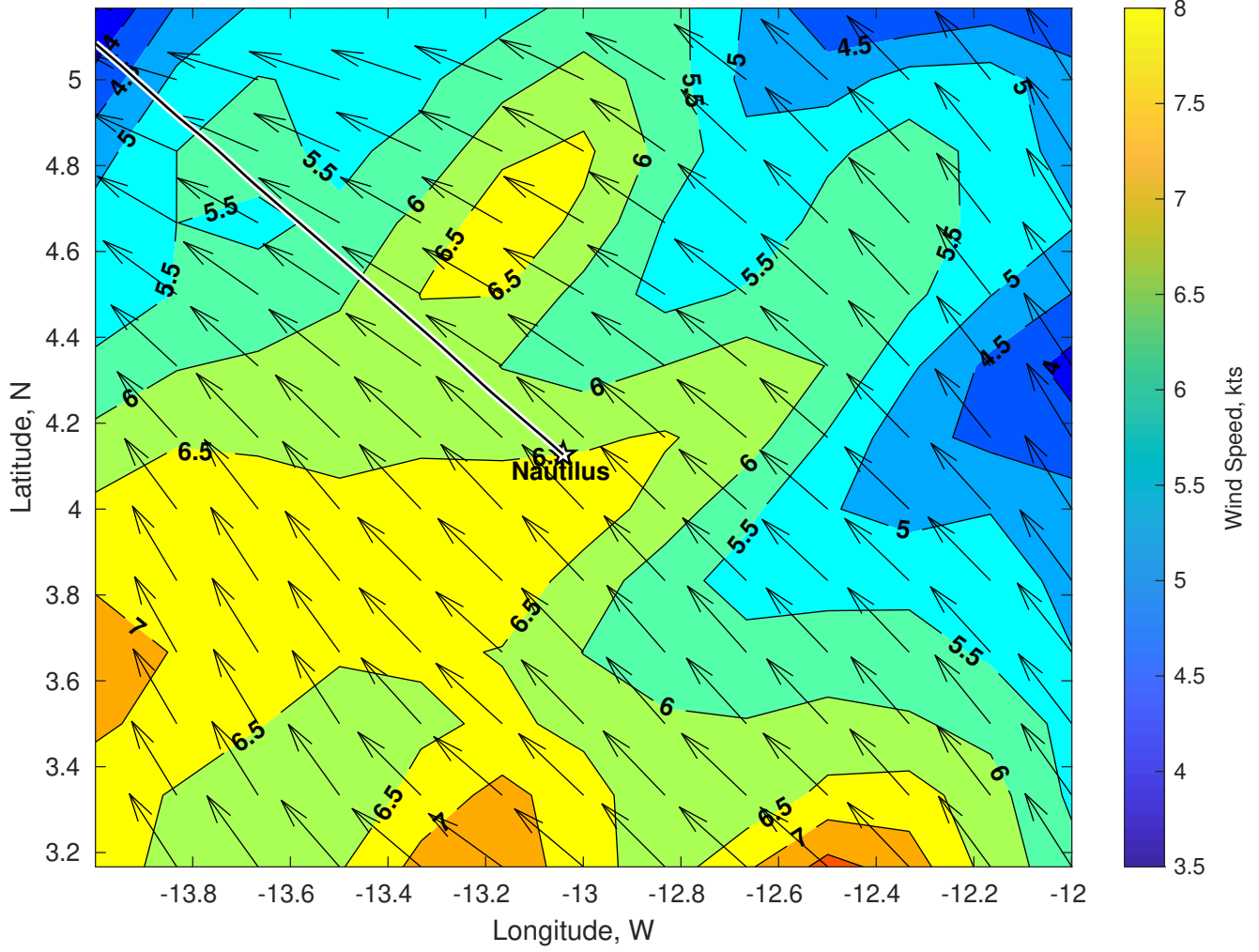
Winds (kts) for Nautilus at 05-Jan-2025 09:00:00
