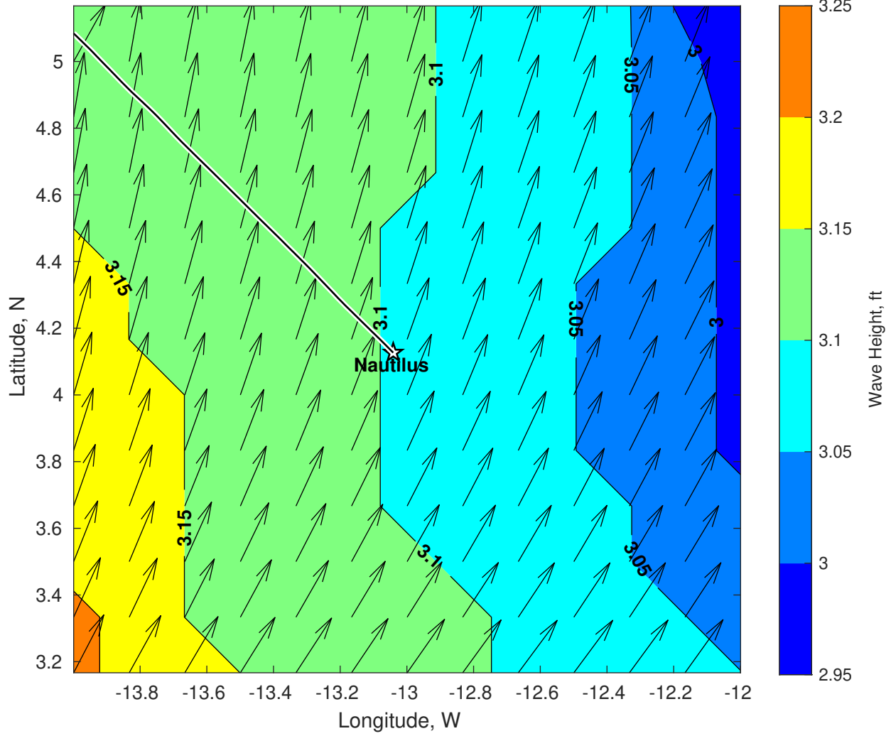
Wave Height (ft) for Nautilus at 05-Jan-2025 09:00:00
