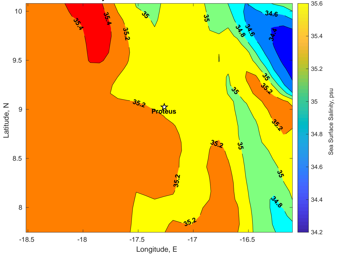
Surface Salinity for Proteus at 04-Jan-2025 00:00:00
