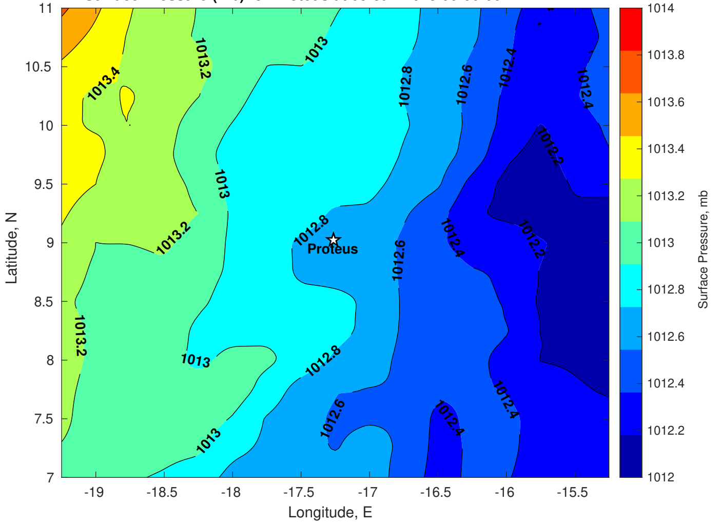
Surface Pressure (mb) for Proteus at 05-Jan-2025 00:00:00
