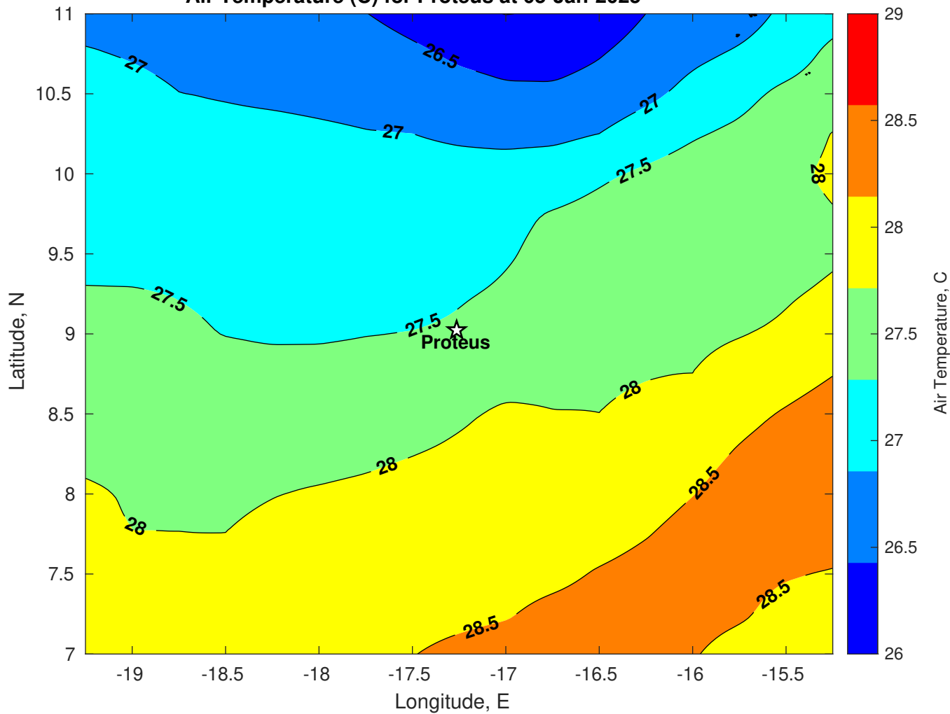
Air Temperature (C) for Proteus at 05-Jan-2025
