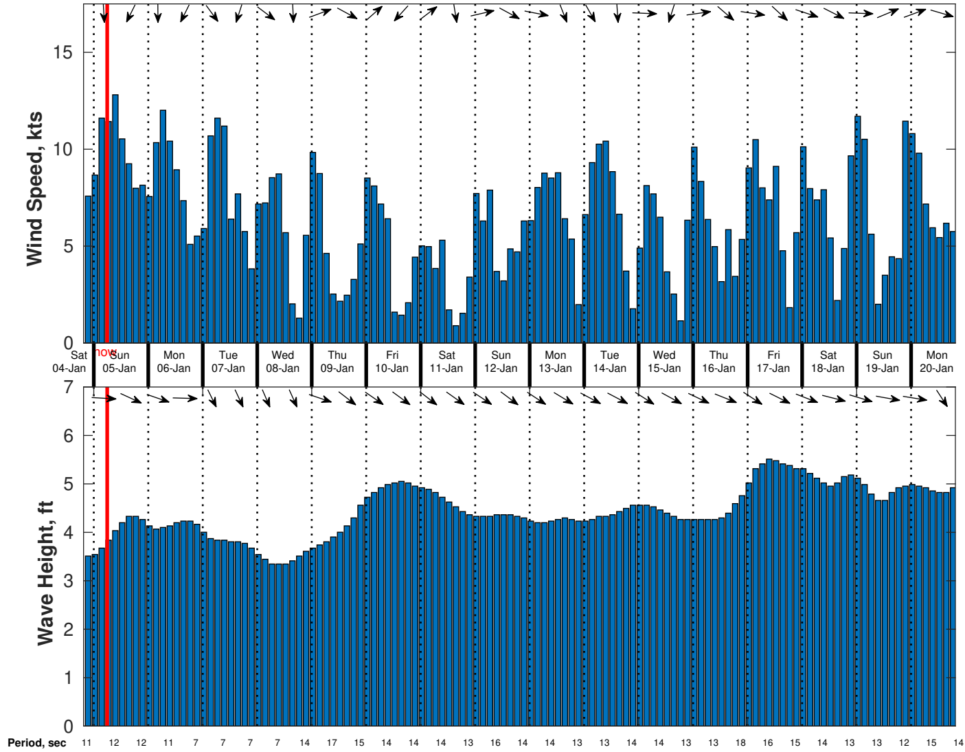
Wind & Wave Forecast for Proteus from 04-Jan-2025 20:00:00 to 20-Jan-2025 20:00:00
