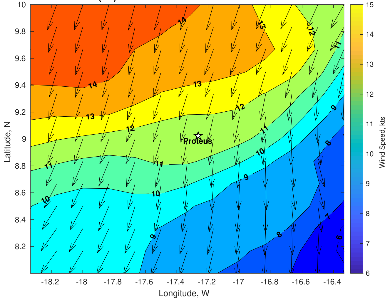
Winds (kts) for Proteus at 05-Jan-2025 09:00:00
