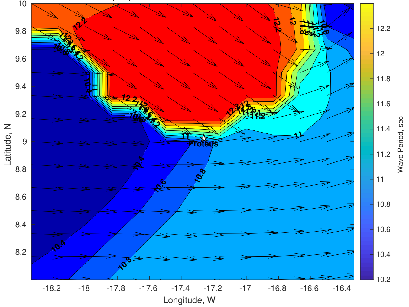
Wave Period (sec) for Proteus at 05-Jan-2025 09:00:00
