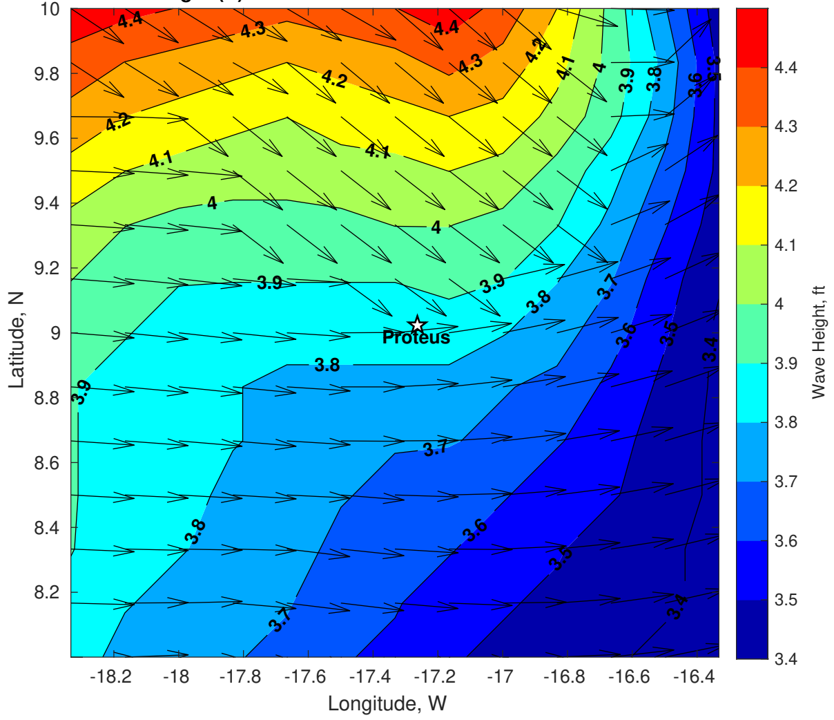
Wave Height (ft) for Proteus at 05-Jan-2025 09:00:00
