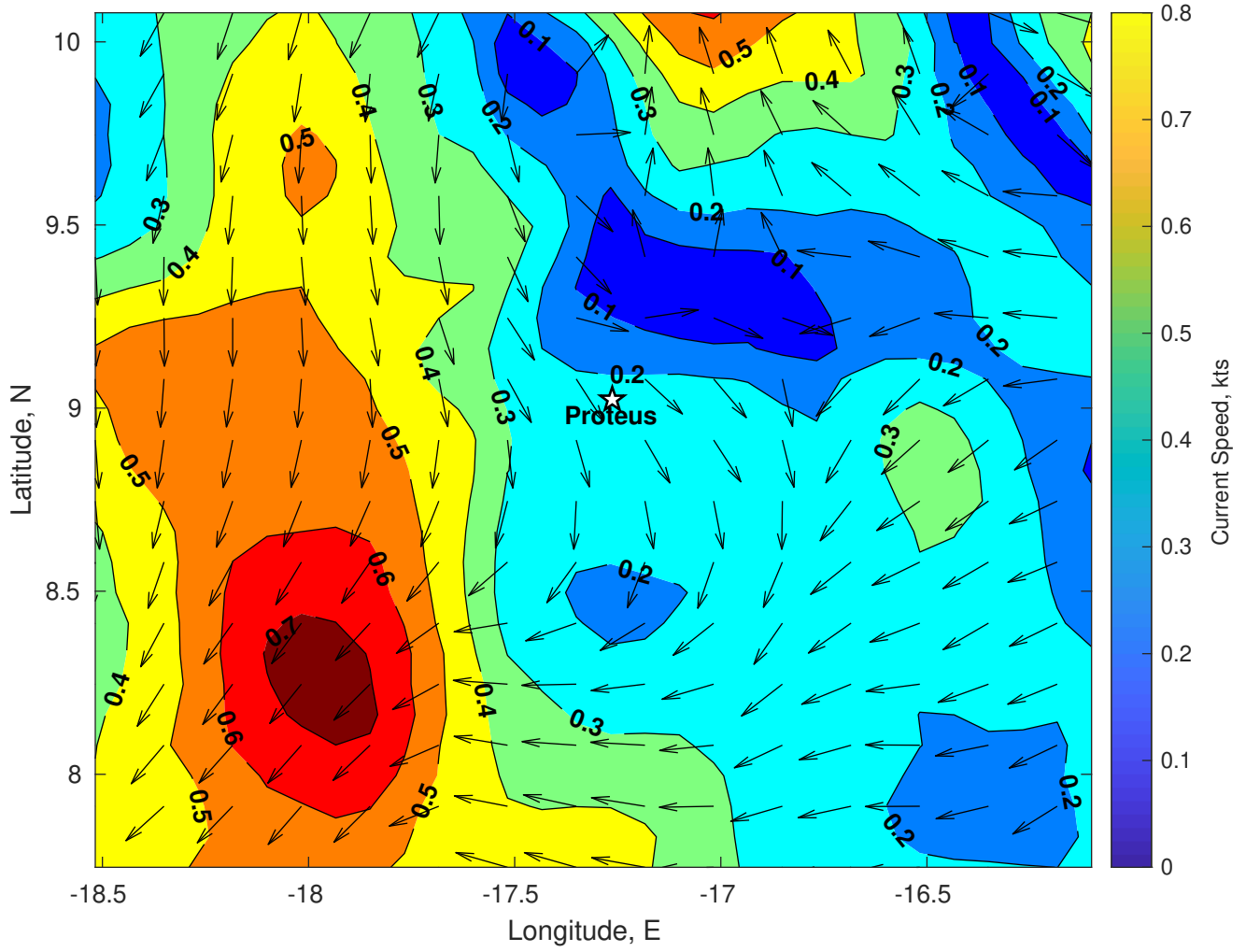
Surface Currents for Proteus at 04-Jan-2025 00:00:00
