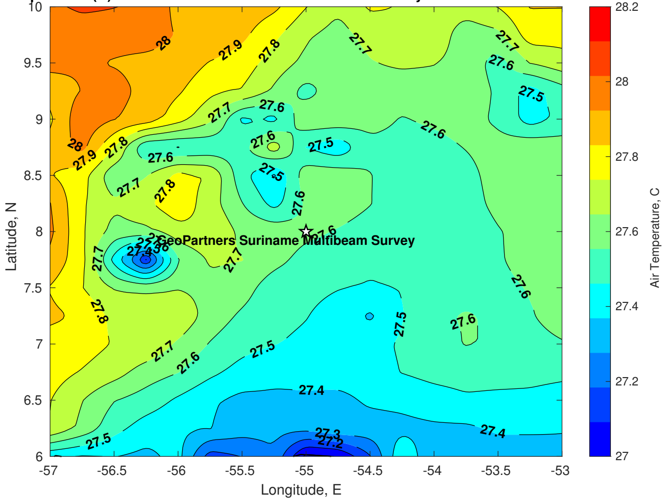
Air Temperature (C) for GeoPartners Suriname Multibeam Survey at 06-Jan-2025
