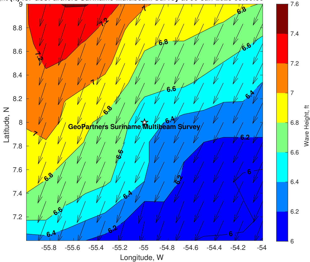
Wave Height (ft) for GeoPartners Suriname Multibeam Survey at 06-Jan-2025 09:00:00
