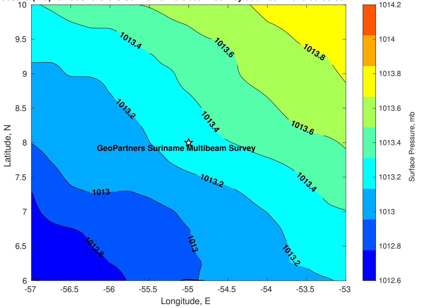
Surface Pressure (mb) for GeoPartners Suriname Multibeam Survey at 07-Jan-2025 00:00:00
