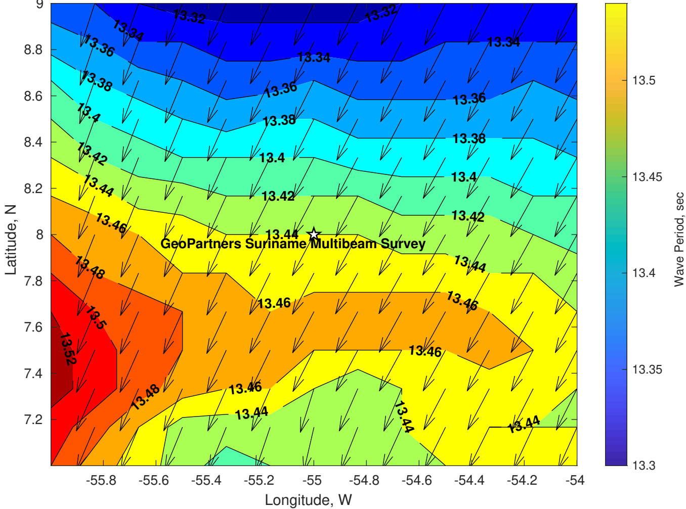
Wave Period (sec) for GeoPartners Suriname Multibeam Survey at 06-Jan-2025 09:00:00
