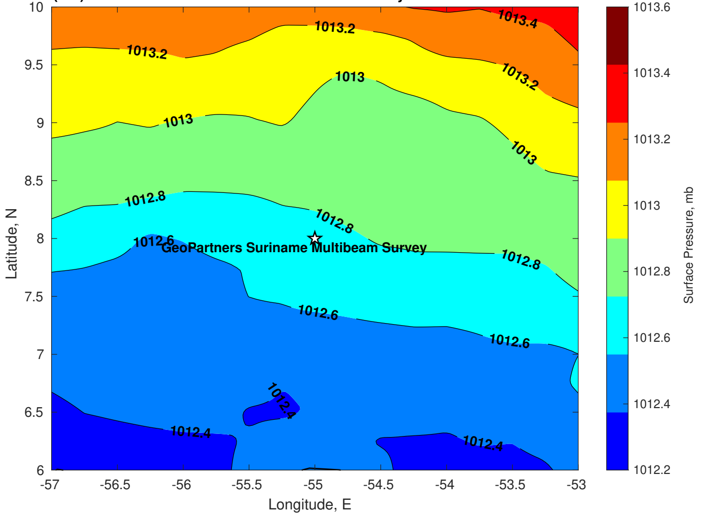
Surface Pressure (mb) for GeoPartners Suriname Multibeam Survey at 06-Jan-2025 00:00:00
