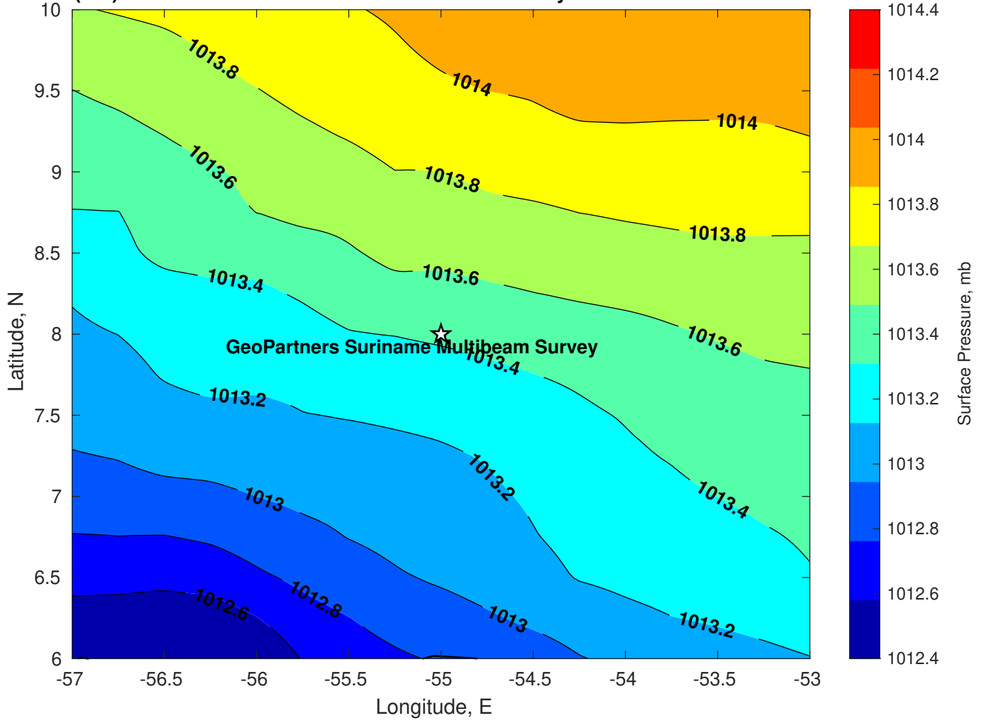
Surface Pressure (mb) for GeoPartners Suriname Multibeam Survey at 08-Jan-2025 00:00:00
