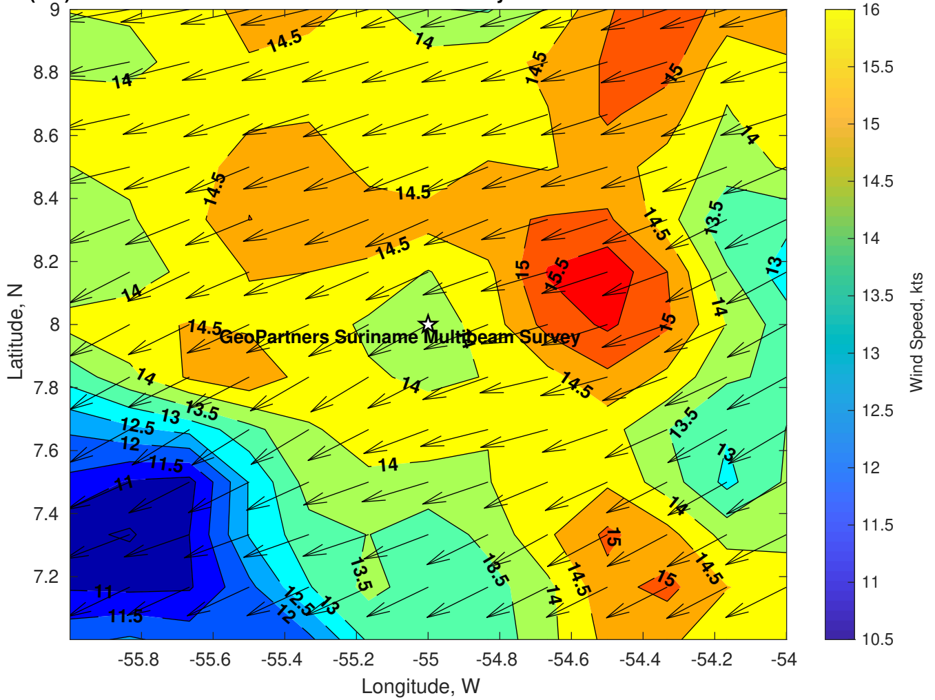
Winds (kts) for GeoPartners Suriname Multibeam Survey at 06-Jan-2025 09:00:00
