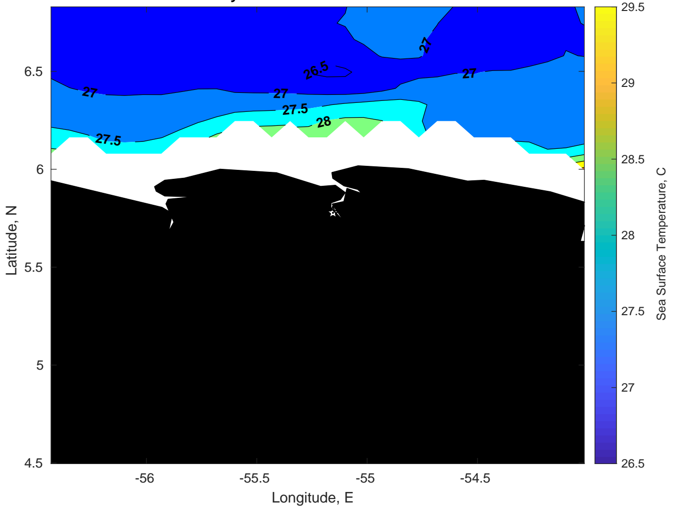
SST for Gyre at 05-Jan-2025 00:00:00
