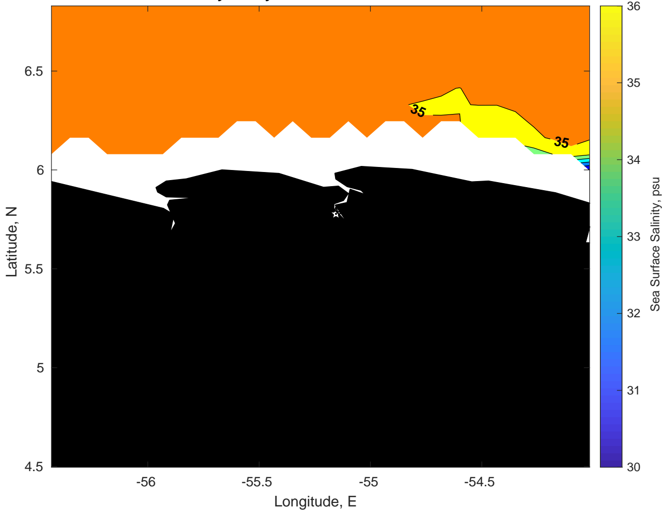
Surface Salinity for Gyre at 05-Jan-2025 00:00:00
