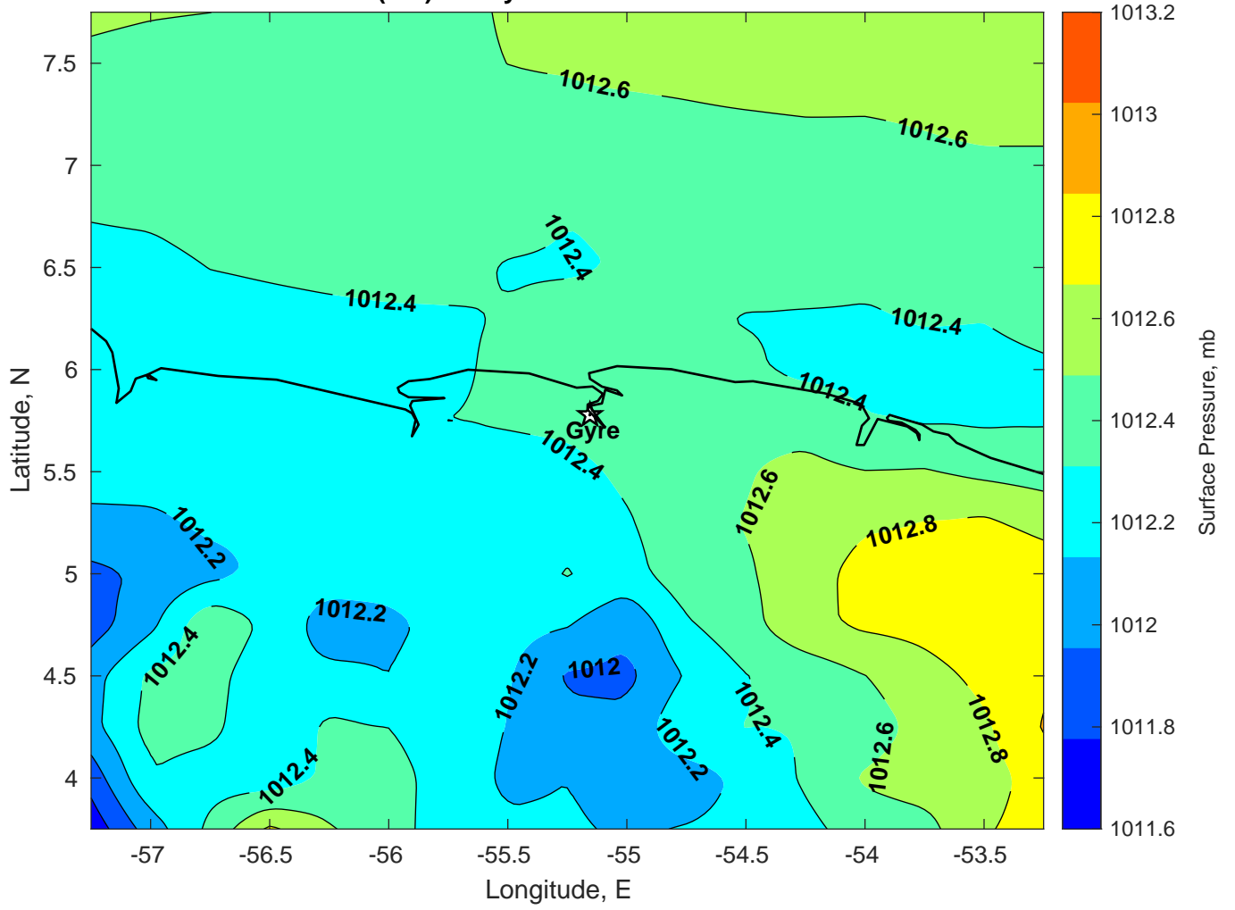
Surface Pressure (mb) for Gyre at 06-Jan-2025 00:00:00
