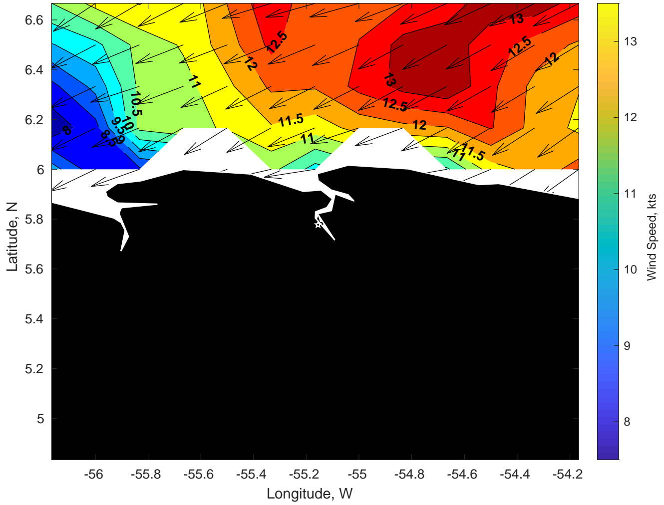
Winds (kts) for Gyre at 06-Jan-2025 09:00:00
