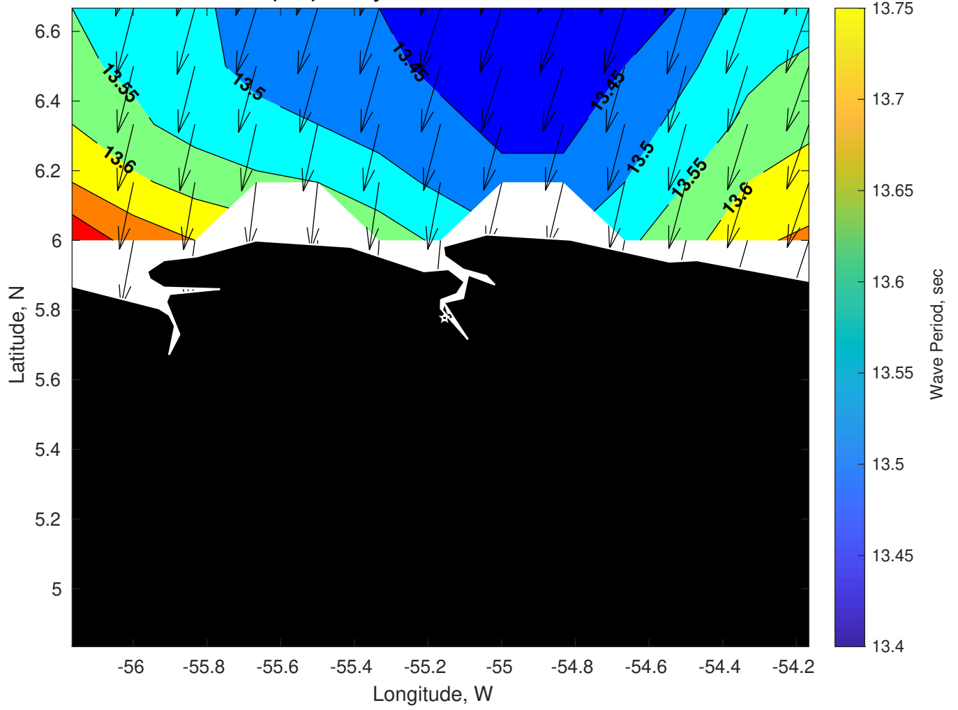
Wave Period (sec) for Gyre at 06-Jan-2025 09:00:00
