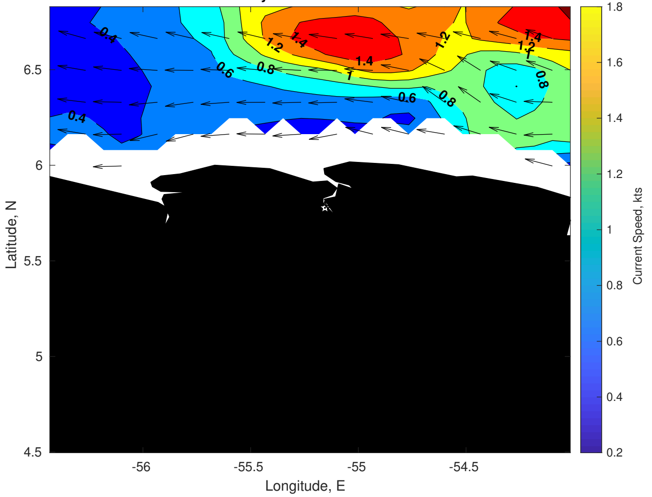
Surface Currents for Gyre at 05-Jan-2025 00:00:00
