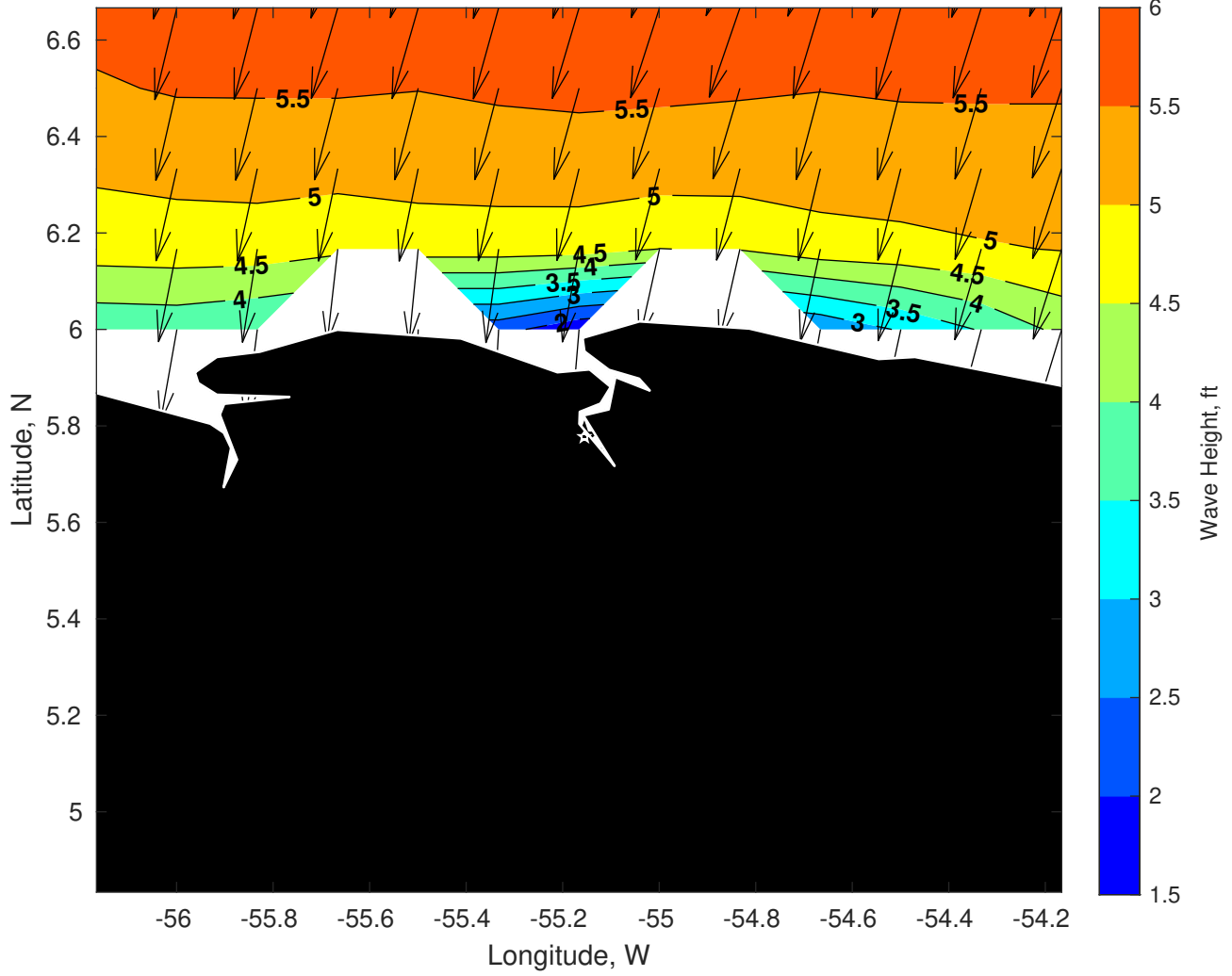
Wave Height (ft) for Gyre at 06-Jan-2025 09:00:00
