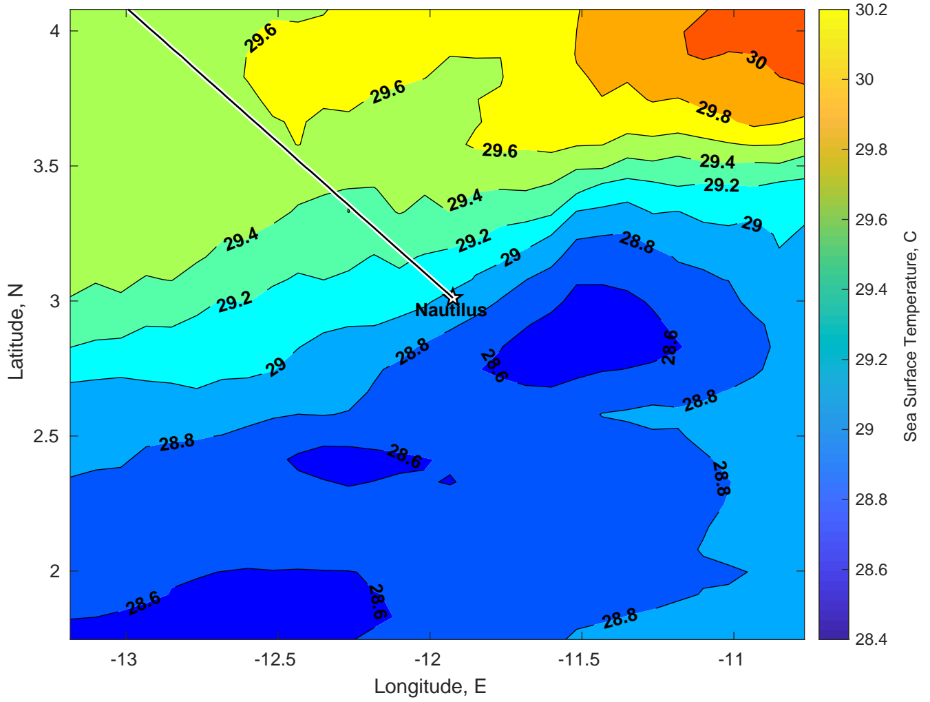
SST for Nautilus at 05-Jan-2025 00:00:00
