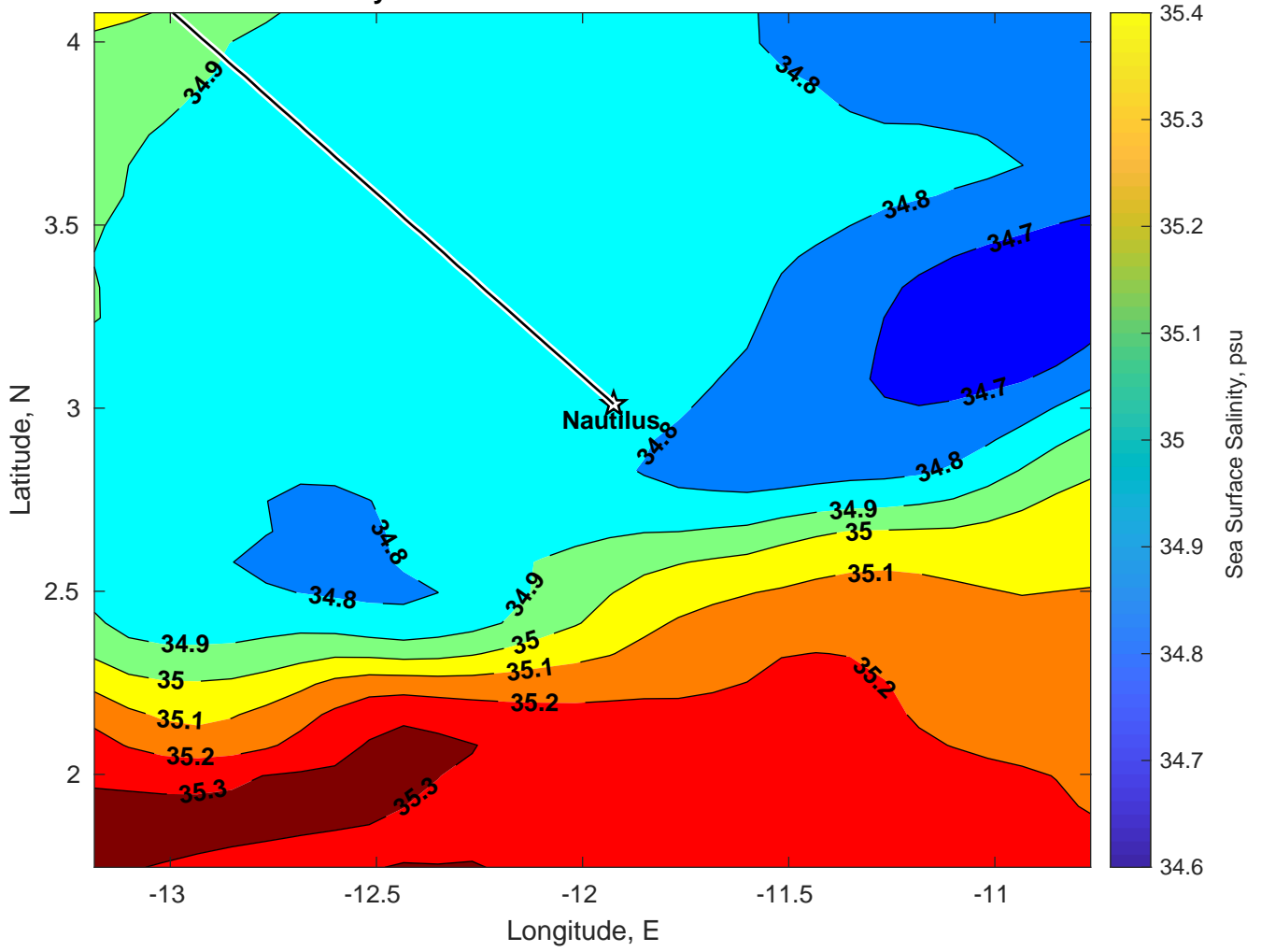
Surface Salinity for Nautilus at 05-Jan-2025 00:00:00
