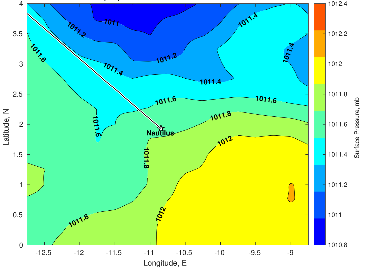
Surface Pressure (mb) for Nautilus at 07-Jan-2025 00:00:00
