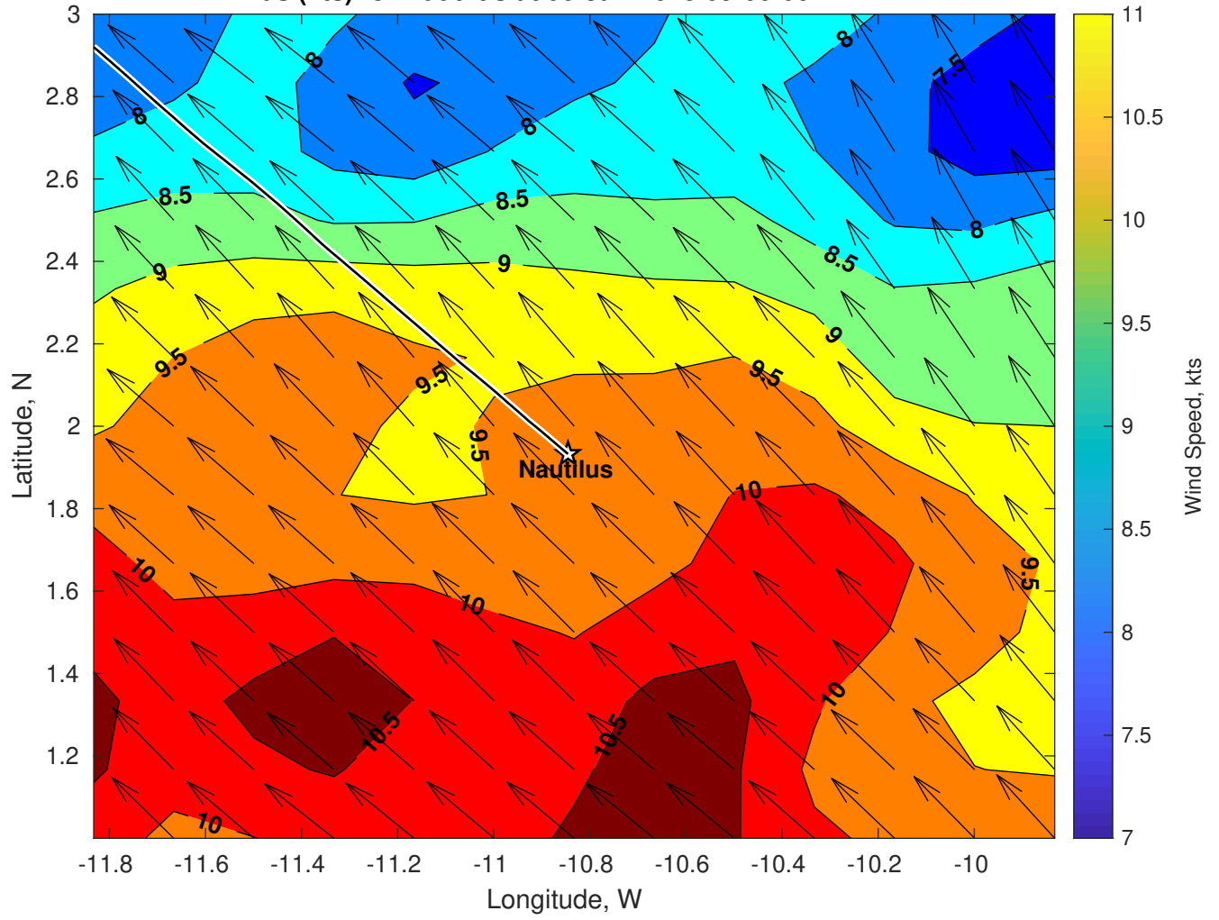
Winds (kts) for Nautilus at 06-Jan-2025 09:00:00
