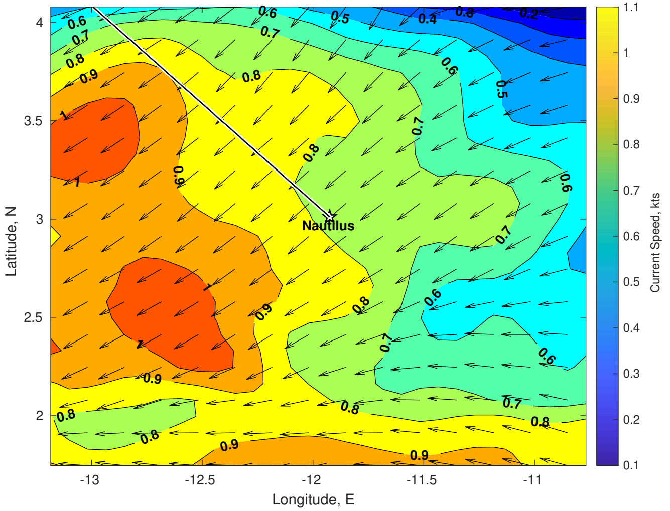
Surface Currents for Nautilus at 05-Jan-2025 00:00:00
