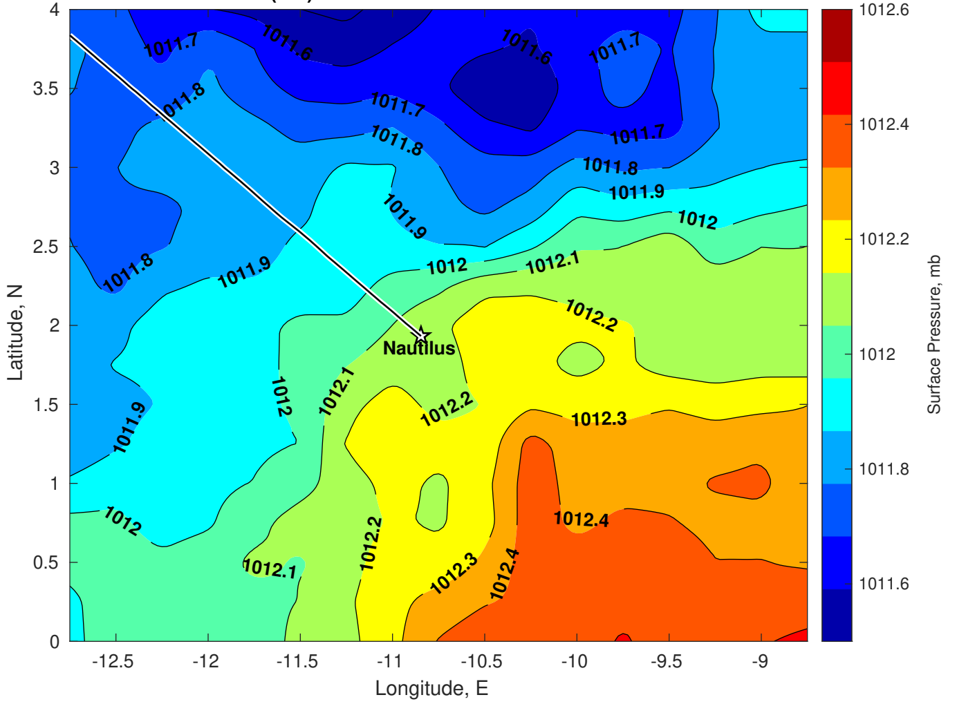
Surface Pressure (mb) for Nautilus at 06-Jan-2025 00:00:00
