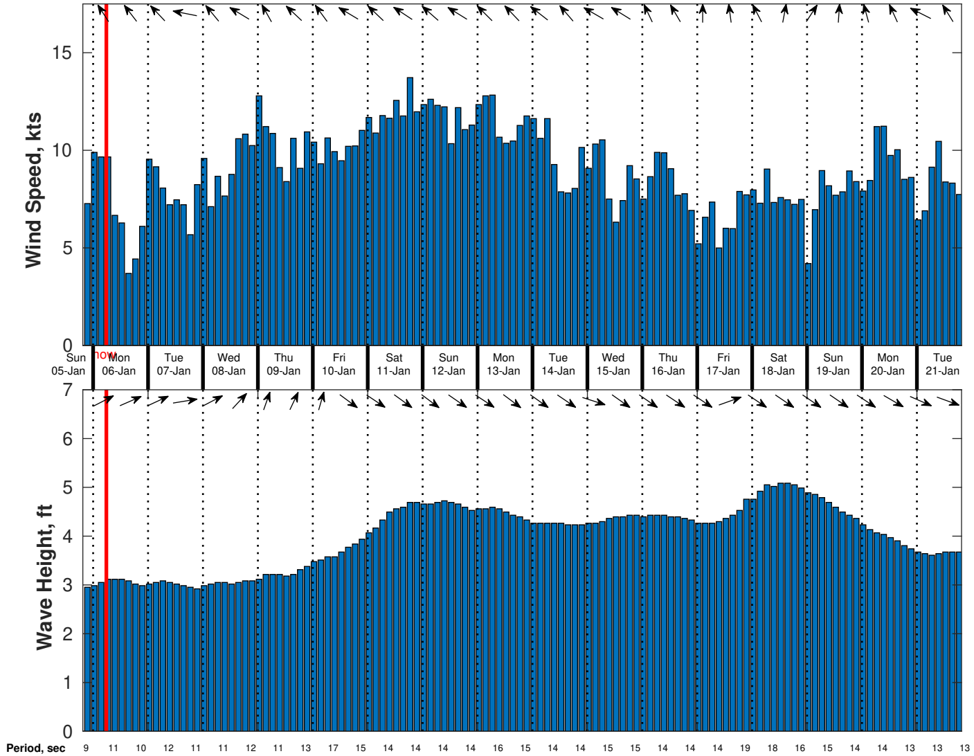
Wind & Wave Forecast for Nautilus from 05-Jan-2025 20:00:00 to 21-Jan-2025 20:00:00
