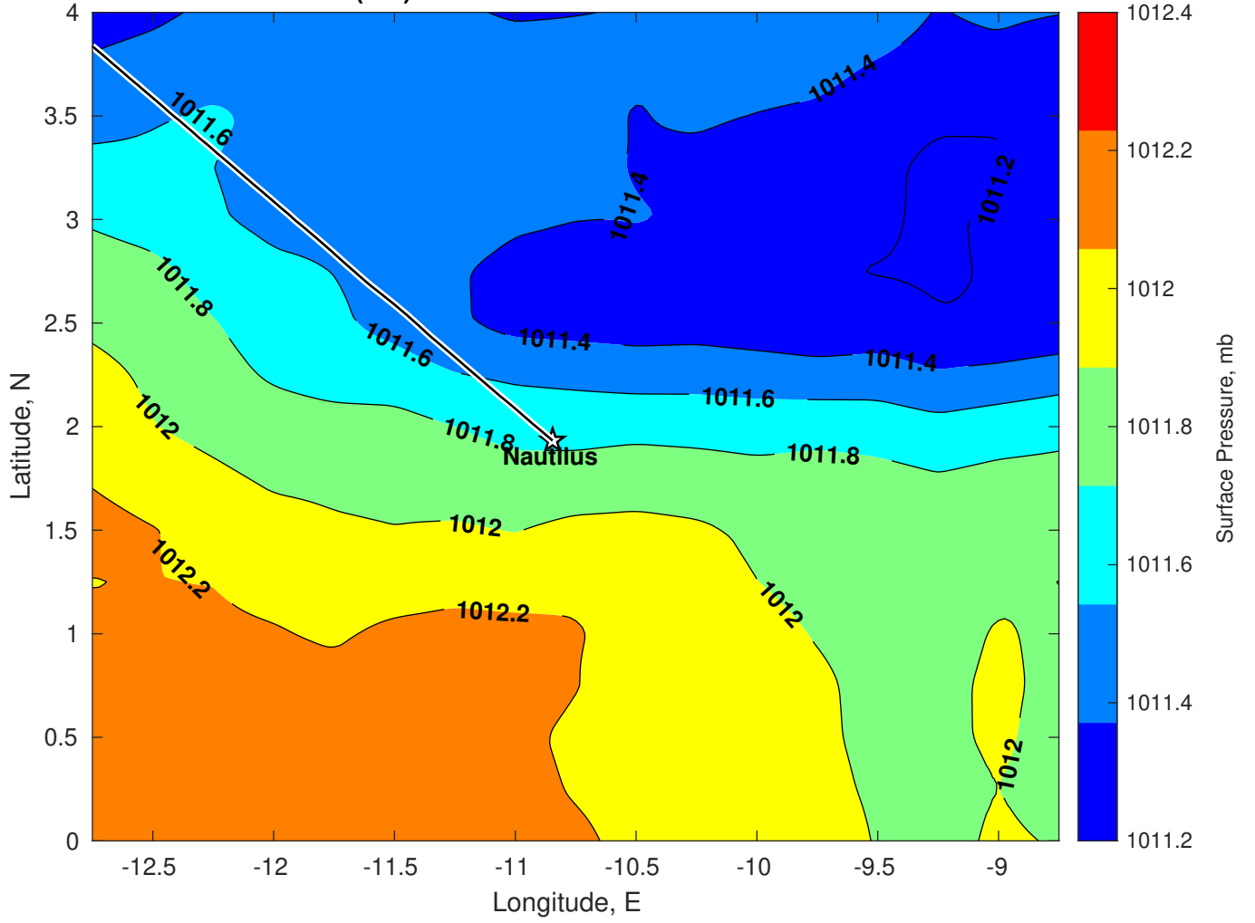
Surface Pressure (mb) for Nautilus at 08-Jan-2025 00:00:00
