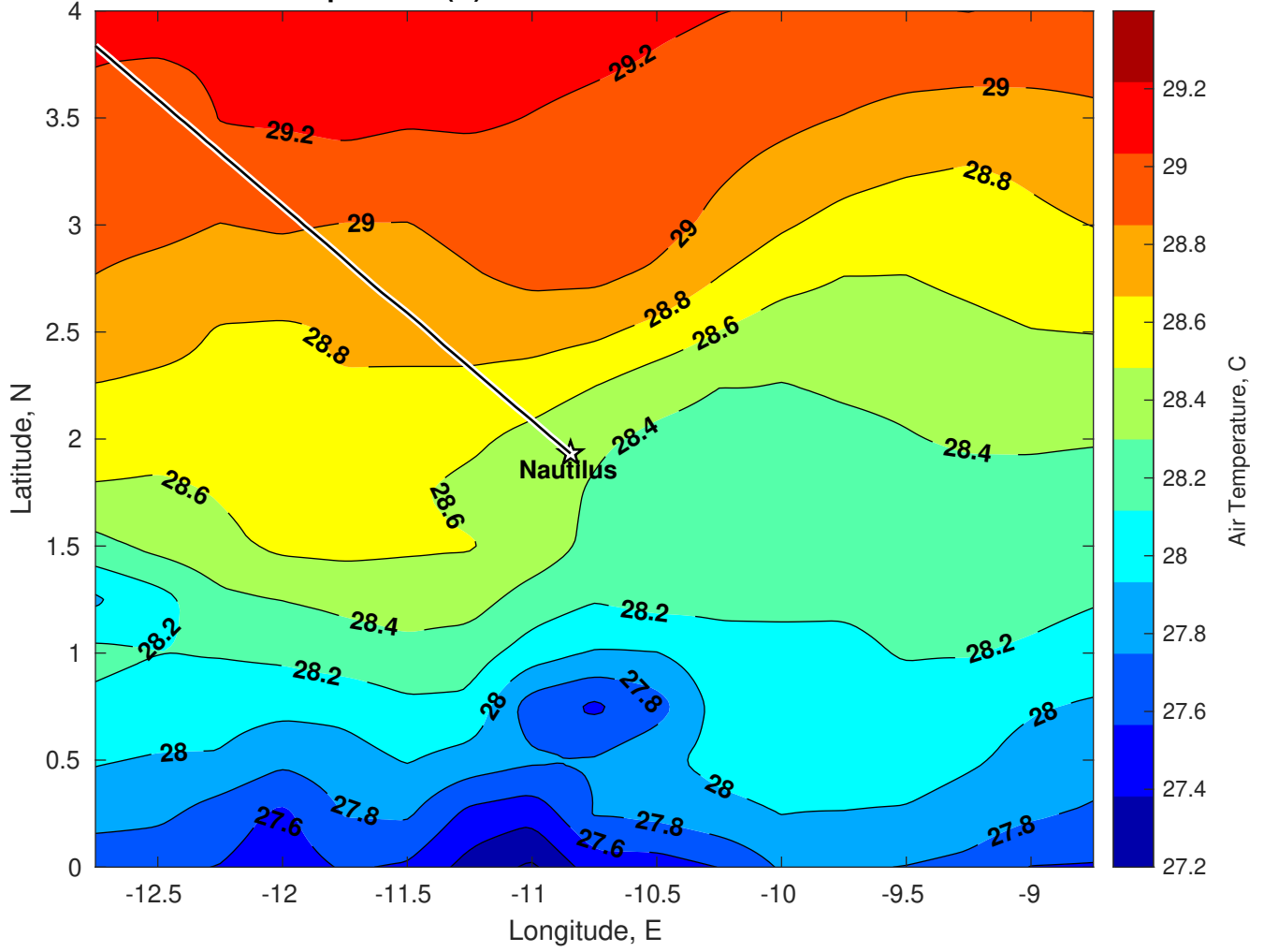
Air Temperature (C) for Nautilus at 06-Jan-2025
