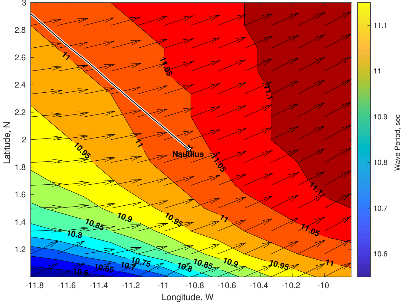
Wave Period (sec) for Nautilus at 06-Jan-2025 09:00:00
