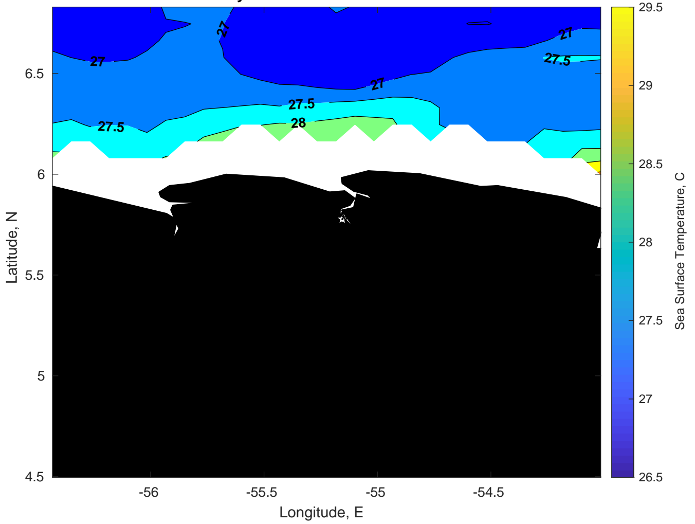
SST for Gyre at 06-Jan-2025 00:00:00
