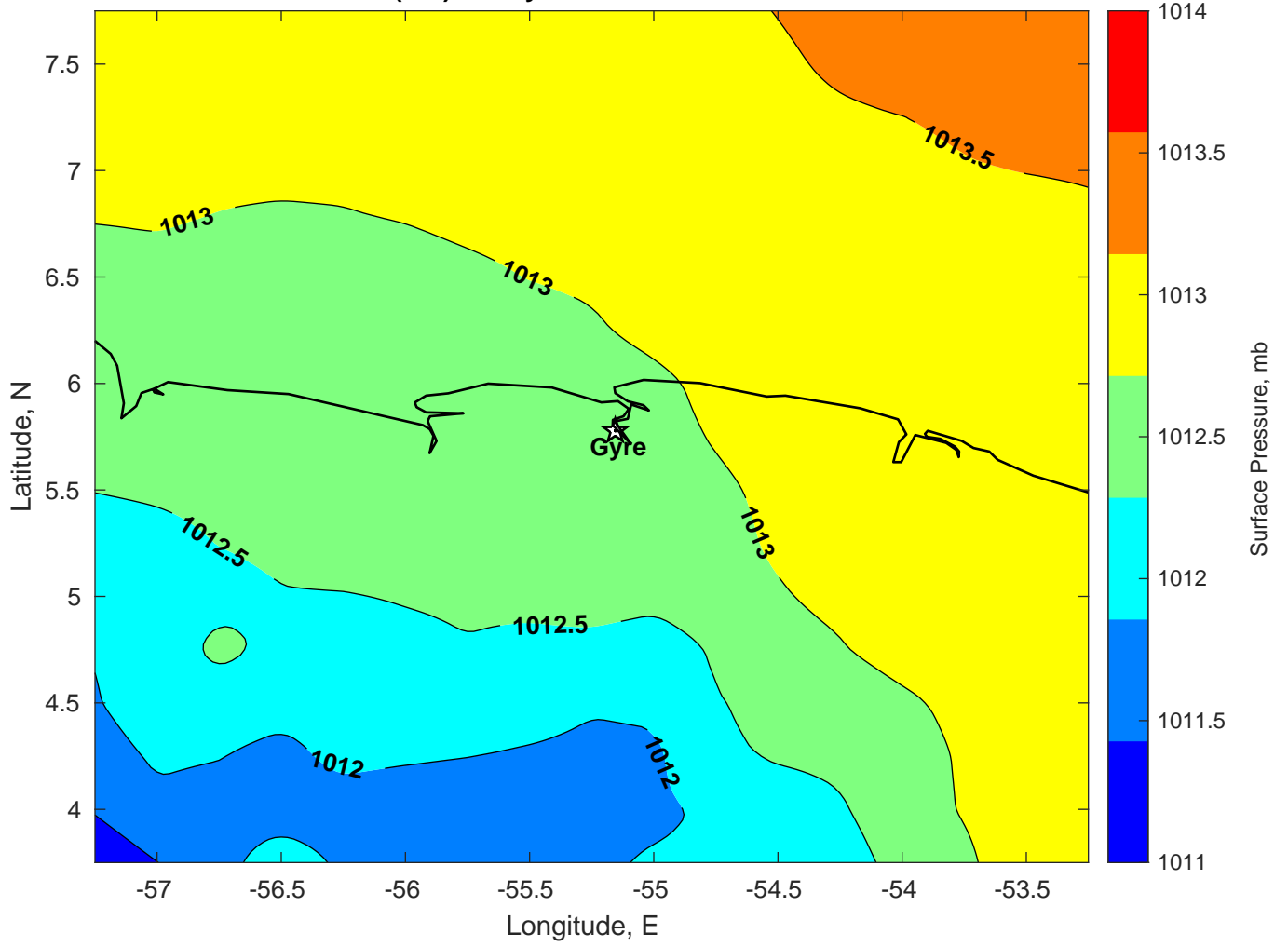
Surface Pressure (mb) for Gyre at 08-Jan-2025 00:00:00
