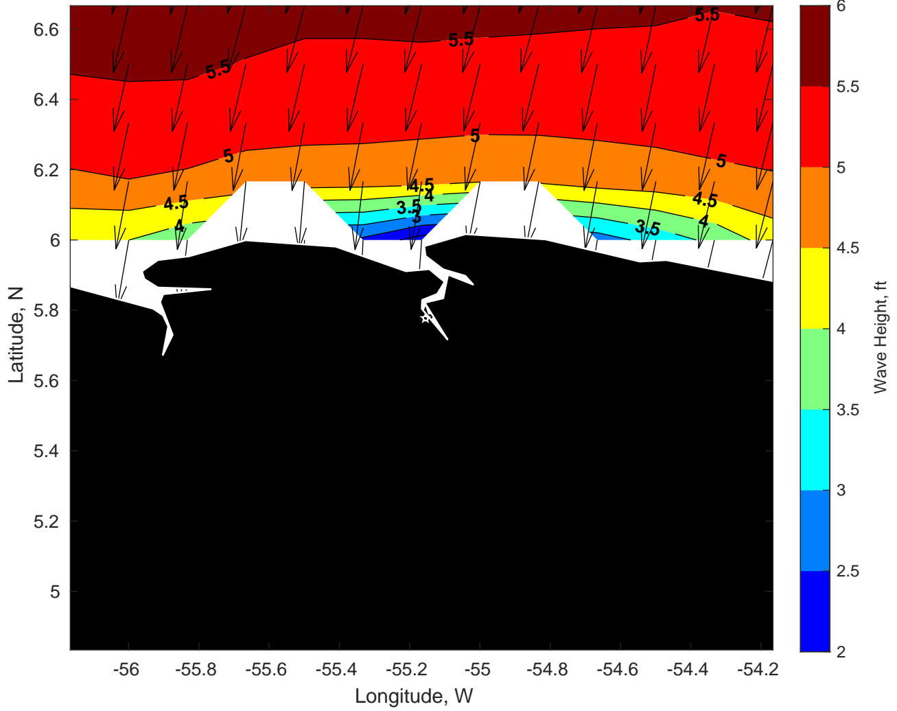
Wave Height (ft) for Gyre at 07-Jan-2025 09:00:00
