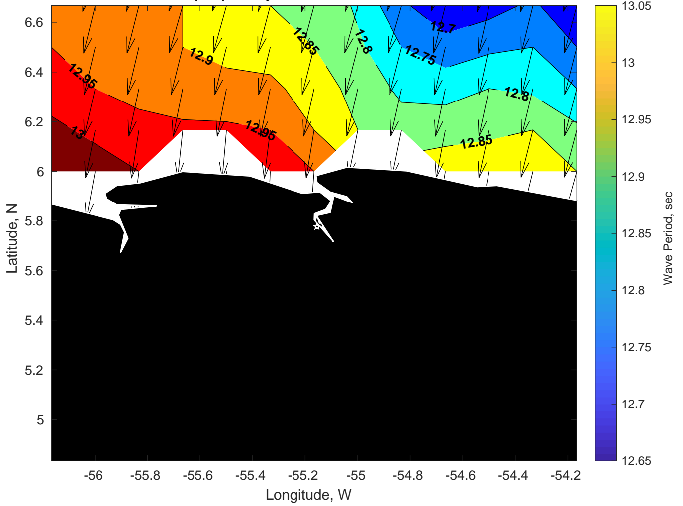
Wave Period (sec) for Gyre at 07-Jan-2025 09:00:00
