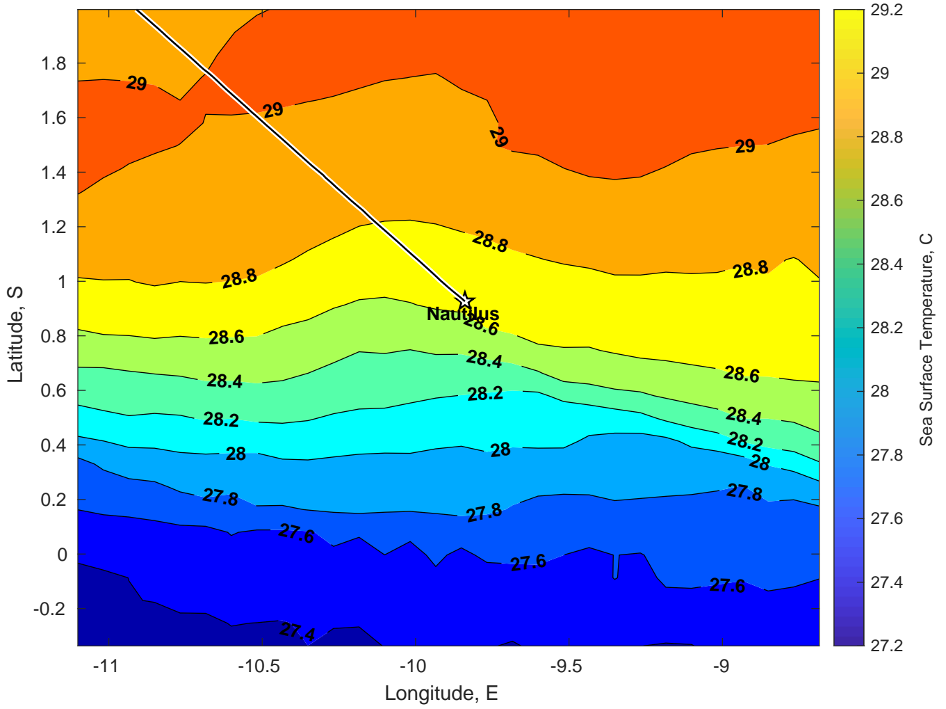
SST for Nautilus at 06-Jan-2025 00:00:00
