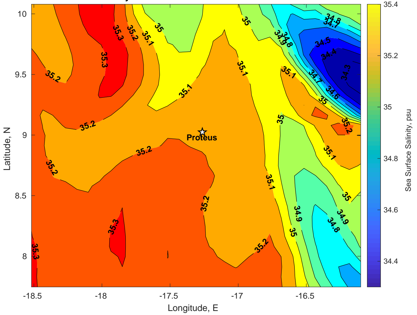
Surface Salinity for Proteus at 06-Jan-2025 00:00:00
