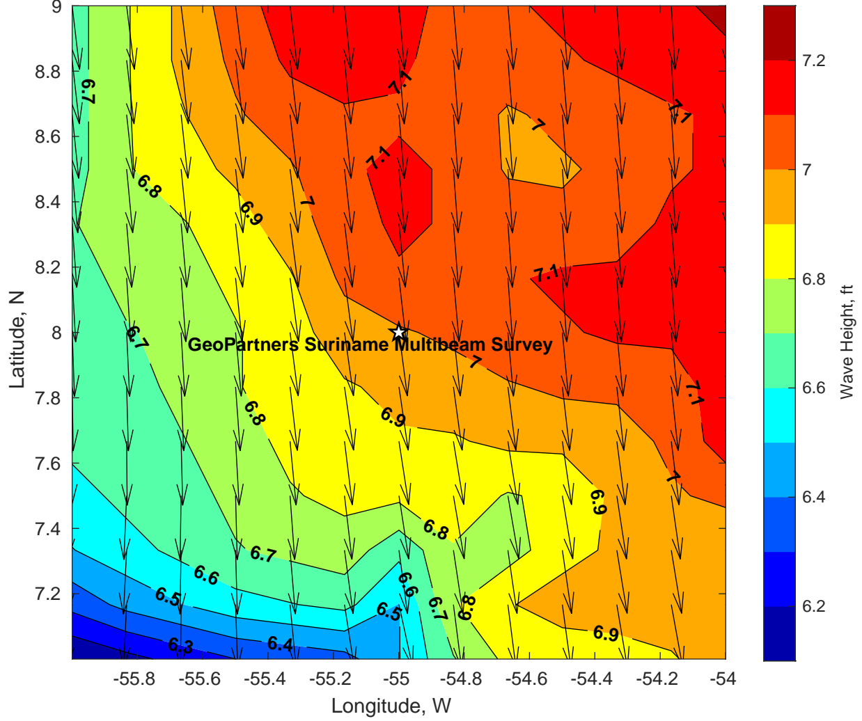
Wave Height (ft) for GeoPartners Suriname Multibeam Survey at 08-Jan-2025 09:00:00
